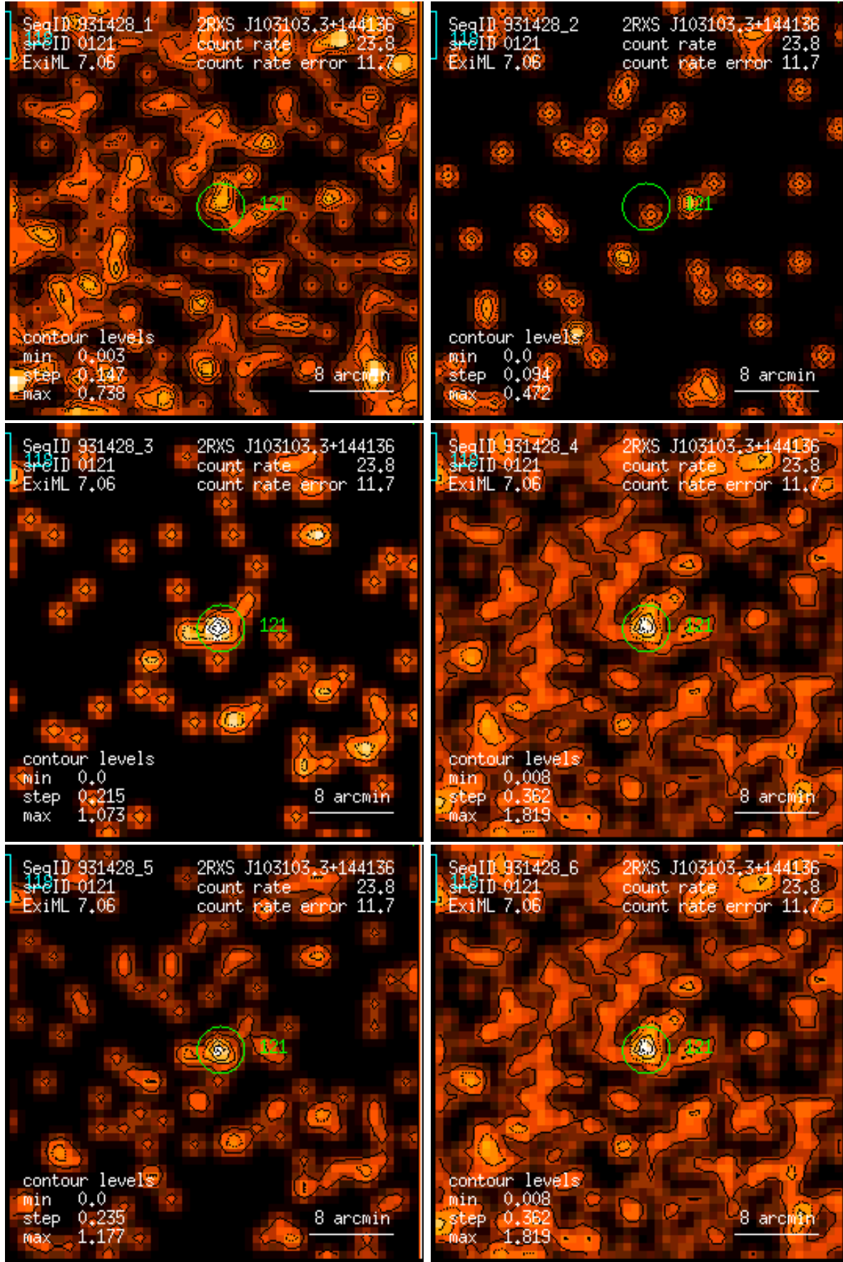
Figure 121: RASS 931428: detection 0121: band rate images, Gaussian filter: (1) PSPC channels 11 – 41, (2) 52 – 90, (3) 91 – 201, (4) 11 – 235, (5) 52 – 201, (6) 11 – 201. Broad band rates in counts/ks. Band rate contour levels in counts/ks/arcmin 2 .
