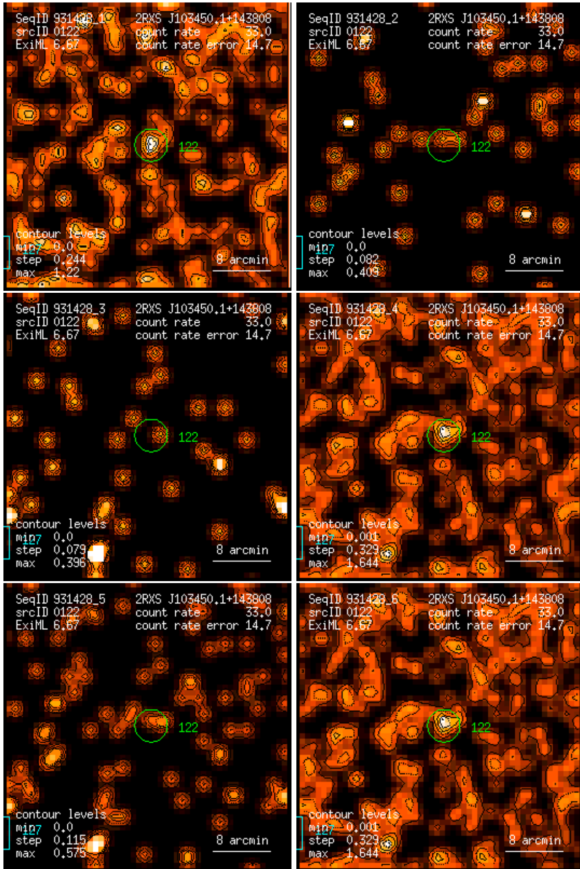
Figure 122: RASS 931428: detection 0122: band rate images, Gaussian filter: (1) PSPC channels 11 – 41, (2) 52 – 90, (3) 91 – 201, (4) 11 – 235, (5) 52 – 201, (6) 11 – 201. Broad band rates in counts/ks. Band rate contour levels in counts/ks/arcmin 2 .
