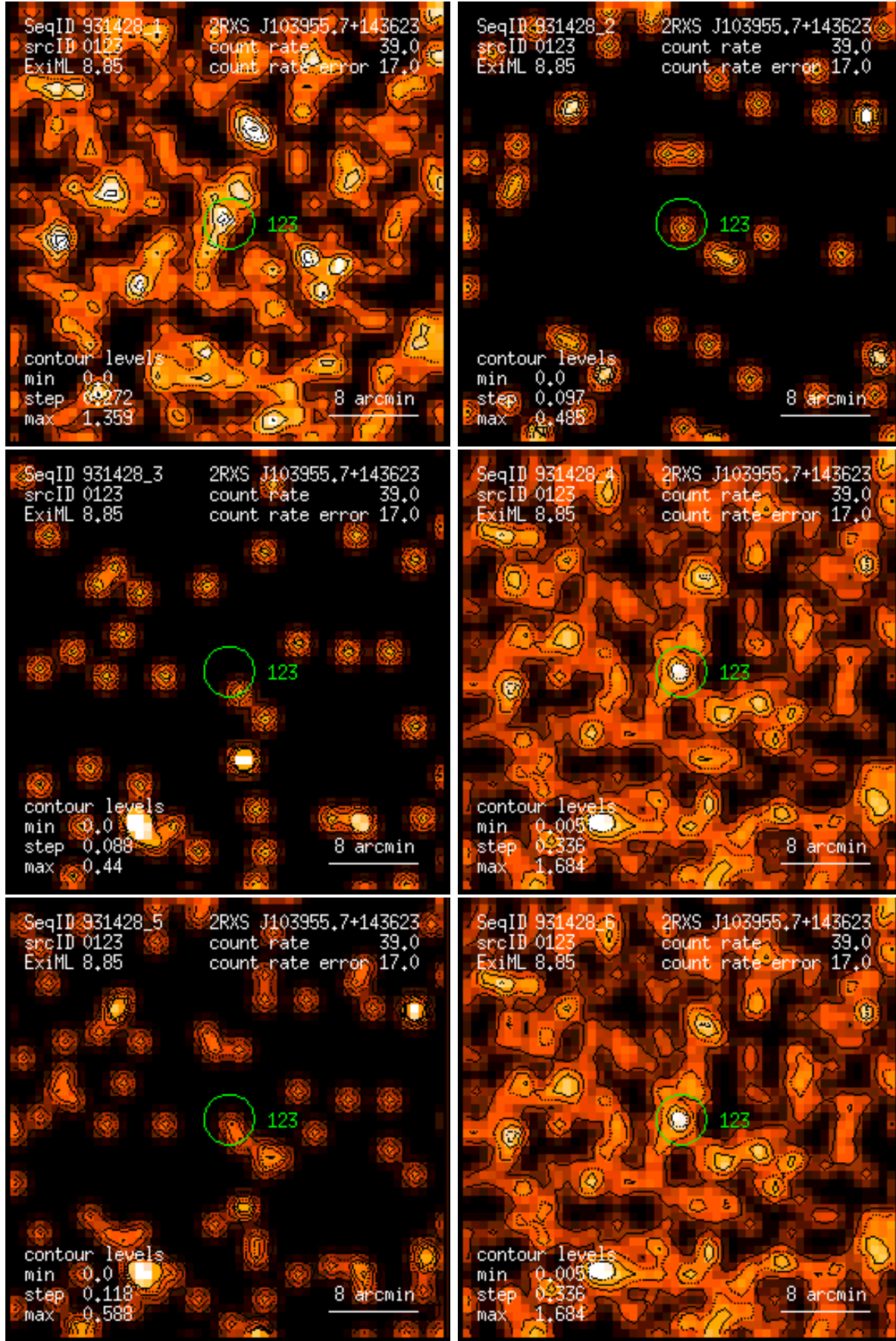
Figure 123: RASS 931428: detection 0123: band rate images, Gaussian filter: (1) PSPC channels 11 – 41, (2) 52 – 90, (3) 91 – 201, (4) 11 – 235, (5) 52 – 201, (6) 11 – 201. Broad band rates in counts/ks. Band rate contour levels in counts/ks/arcmin 2 .
