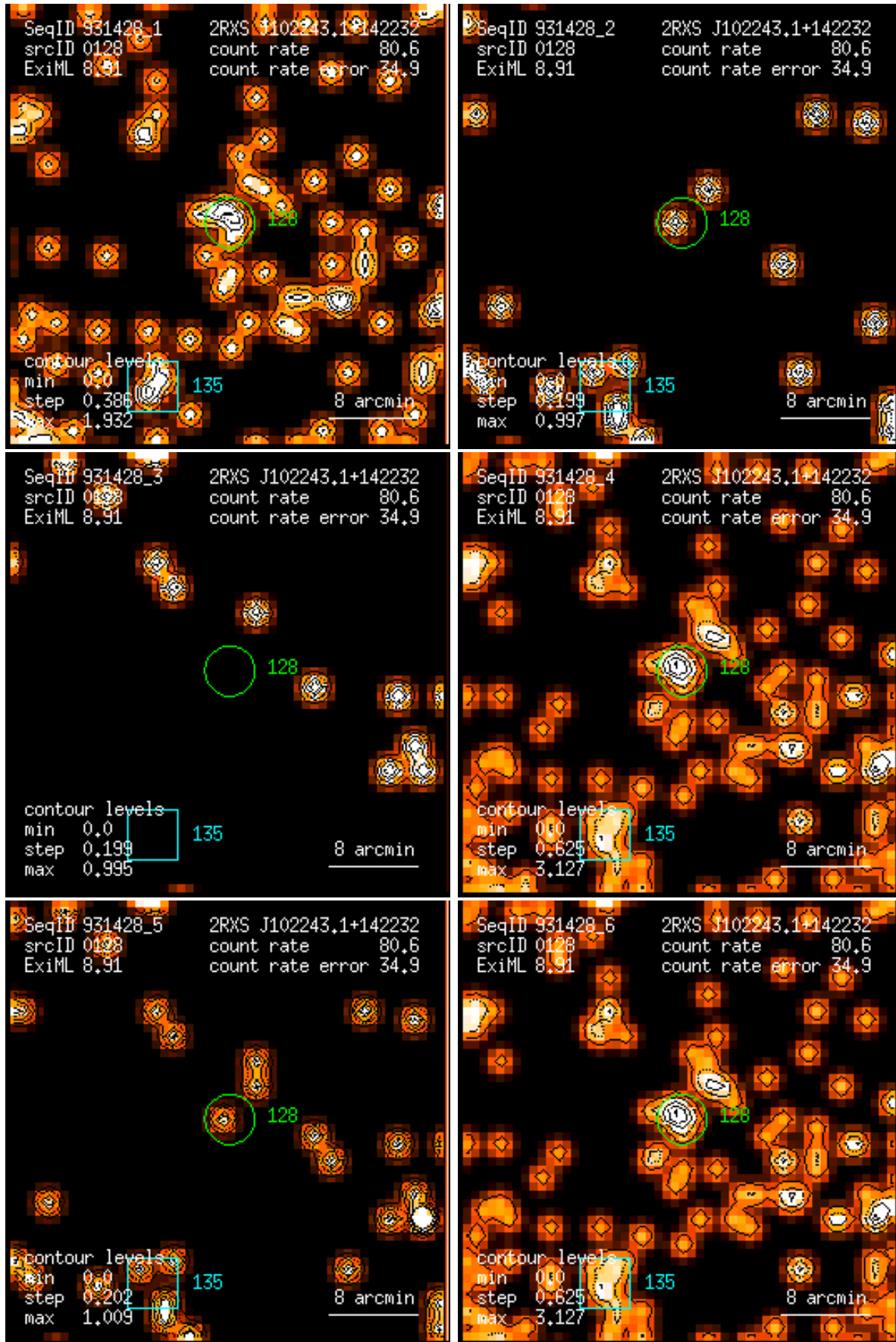
Figure 128: RASS 931428: detection 0128: band rate images, Gaussian filter: (1) PSPC channels 11 – 41, (2) 52 – 90, (3) 91 – 201, (4) 11 – 235, (5) 52 – 201, (6) 11 – 201. Broad band rates in counts/ks. Band rate contour levels in counts/ks/arcmin 2 .
