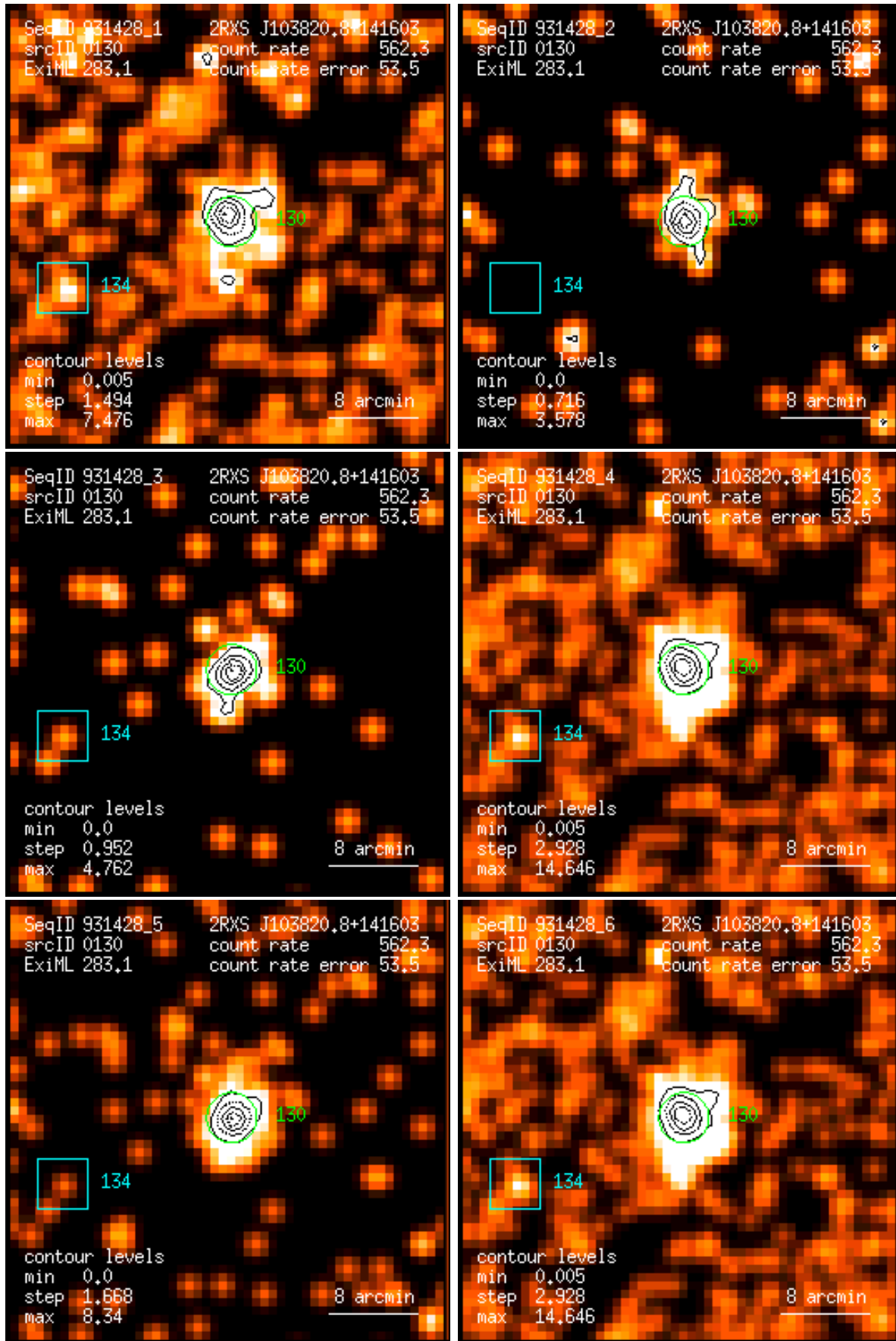
Figure 130: RASS 931428: detection 0130: band rate images, Gaussian filter: (1) PSPC channels 11 – 41, (2) 52 – 90, (3) 91 – 201, (4) 11 – 235, (5) 52 – 201, (6) 11 – 201. Broad band rates in counts/ks. Band rate contour levels in counts/ks/arcmin 2 .
