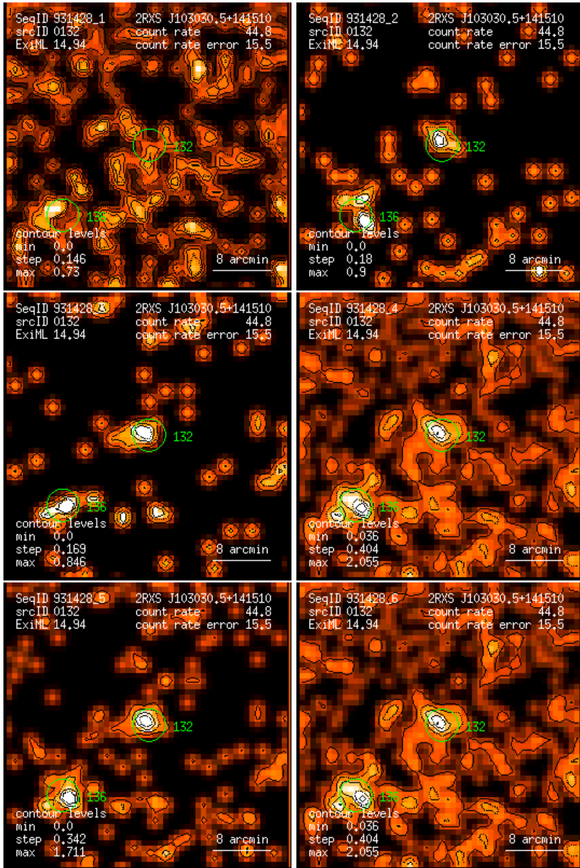
Figure 132: RASS 931428: detection 0132: band rate images, Gaussian filter: (1) PSPC channels 11 – 41, (2) 52 – 90, (3) 91 – 201, (4) 11 – 235, (5) 52 – 201, (6) 11 – 201. Broad band rates in counts/ks. Band rate contour levels in counts/ks/arcmin 2 .
