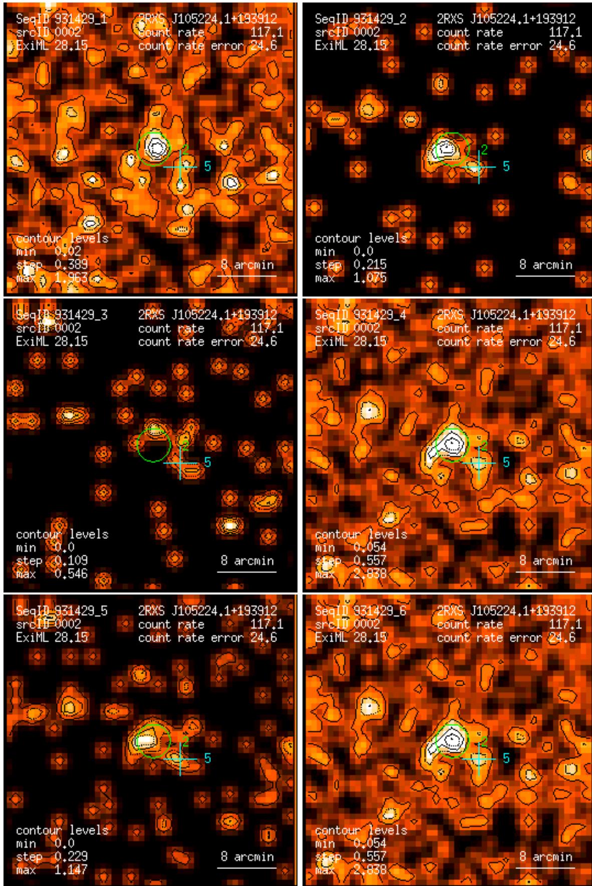
Figure 2: RASS 931429: detection 0002: band rate images, Gaussian filter: (1) PSPC channels 11 – 41, (2) 52 – 90, (3) 91 – 201, (4) 11 – 235, (5) 52 – 201, (6) 11 – 201. Broad band rates in counts/ks. Band rate contour levels in counts/ks/arcmin 2 .
