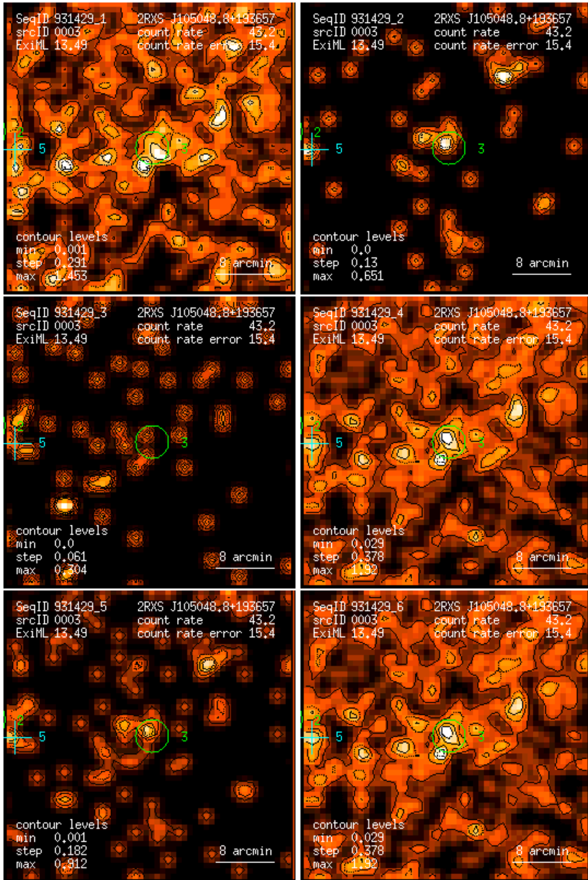
Figure 3: RASS 931429: detection 0003: band rate images, Gaussian filter: (1) PSPC channels 11 – 41, (2) 52 – 90, (3) 91 – 201, (4) 11 – 235, (5) 52 – 201, (6) 11 – 201. Broad band rates in counts/ks. Band rate contour levels in counts/ks/arcmin 2 .
