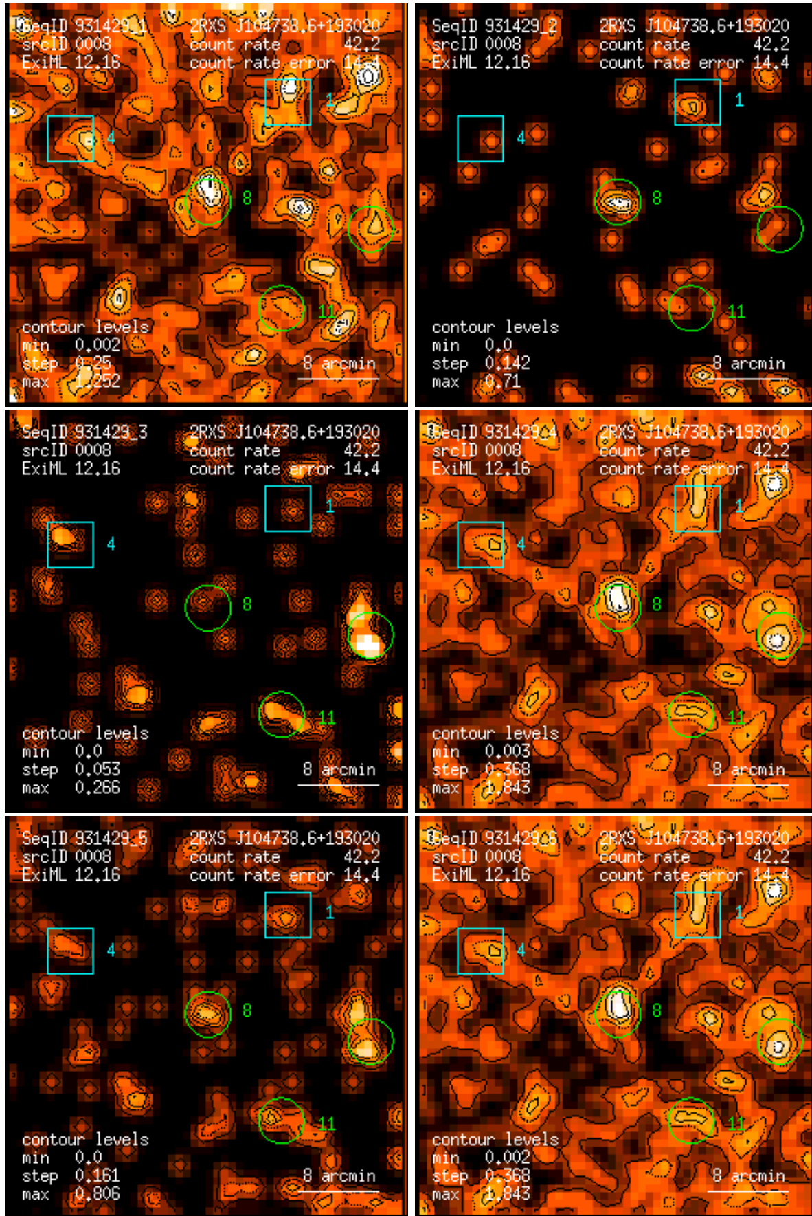
Figure 8: RASS 931429: detection 0008: band rate images, Gaussian filter: (1) PSPC channels 11 – 41, (2) 52 – 90, (3) 91 – 201, (4) 11 – 235, (5) 52 – 201, (6) 11 – 201. Broad band rates in counts/ks. Band rate contour levels in counts/ks/arcmin 2 .
