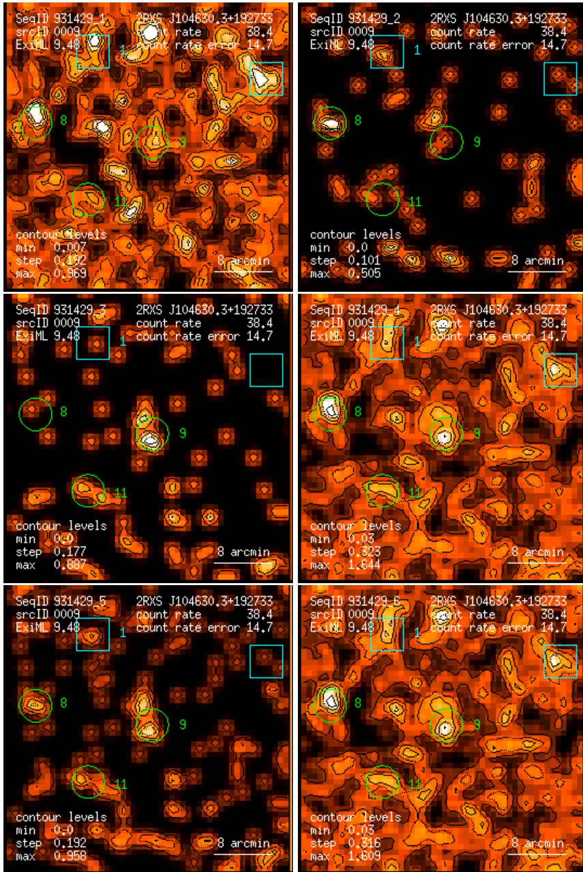
Figure 9: RASS 931429: detection 0009: band rate images, Gaussian filter: (1) PSPC channels 11 – 41, (2) 52 – 90, (3) 91 – 201, (4) 11 – 235, (5) 52 – 201, (6) 11 – 201. Broad band rates in counts/ks. Band rate contour levels in counts/ks/arcmin 2 .
