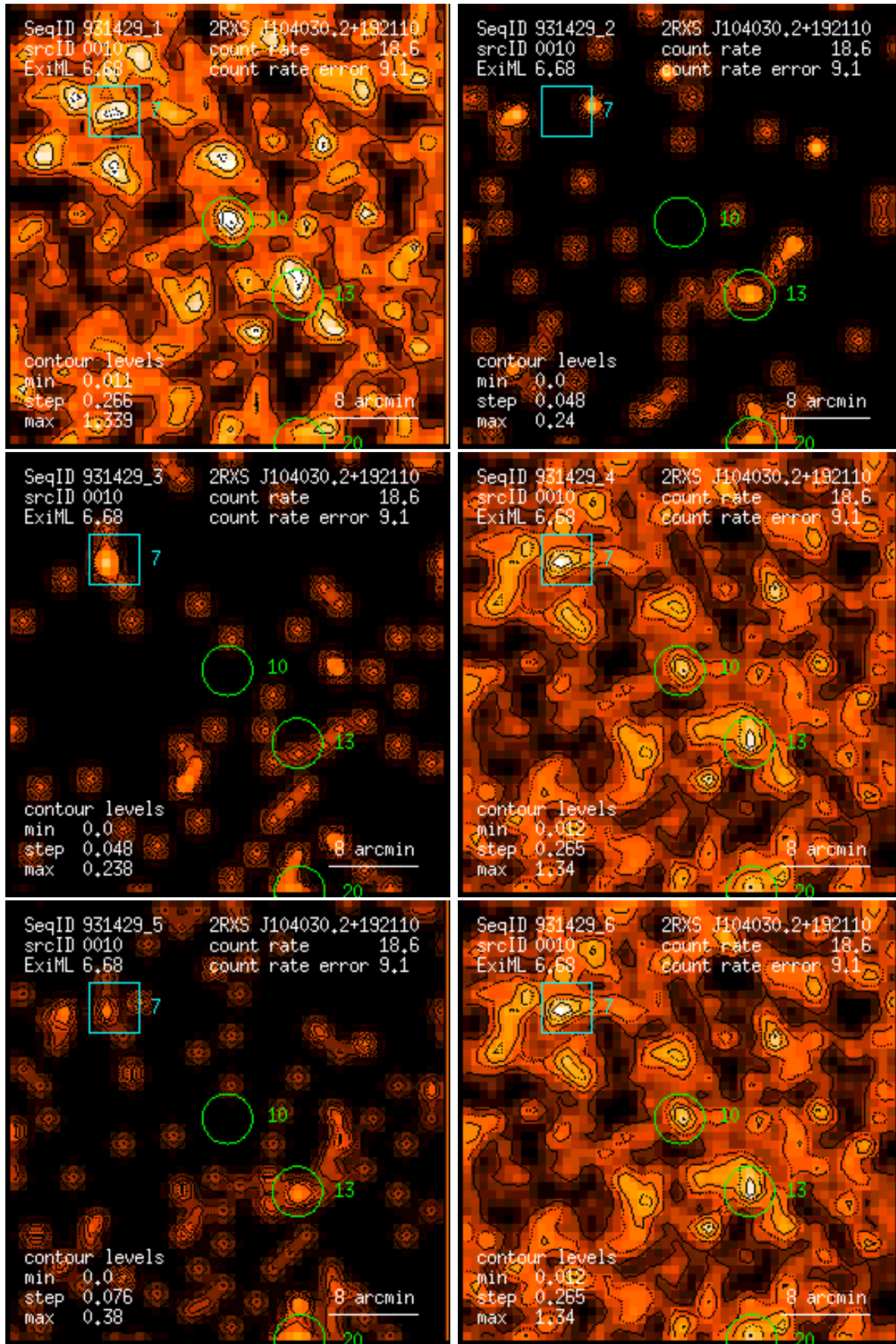
Figure 10: RASS 931429: detection 0010: band rate images, Gaussian filter: (1) PSPC channels 11 – 41, (2) 52 – 90, (3) 91 – 201, (4) 11 – 235, (5) 52 – 201, (6) 11 – 201. Broad band rates in counts/ks. Band rate contour levels in counts/ks/arcmin 2 .
