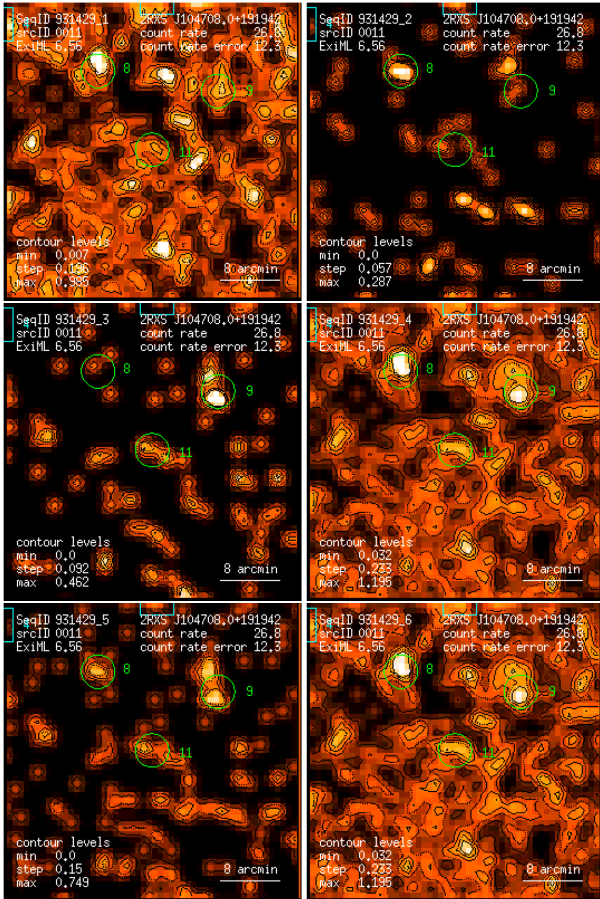
Figure 11: RASS 931429: detection 0011: band rate images, Gaussian filter: (1) PSPC channels 11 – 41, (2) 52 – 90, (3) 91 – 201, (4) 11 – 235, (5) 52 – 201, (6) 11 – 201. Broad band rates in counts/ks. Band rate contour levels in counts/ks/arcmin 2 .
