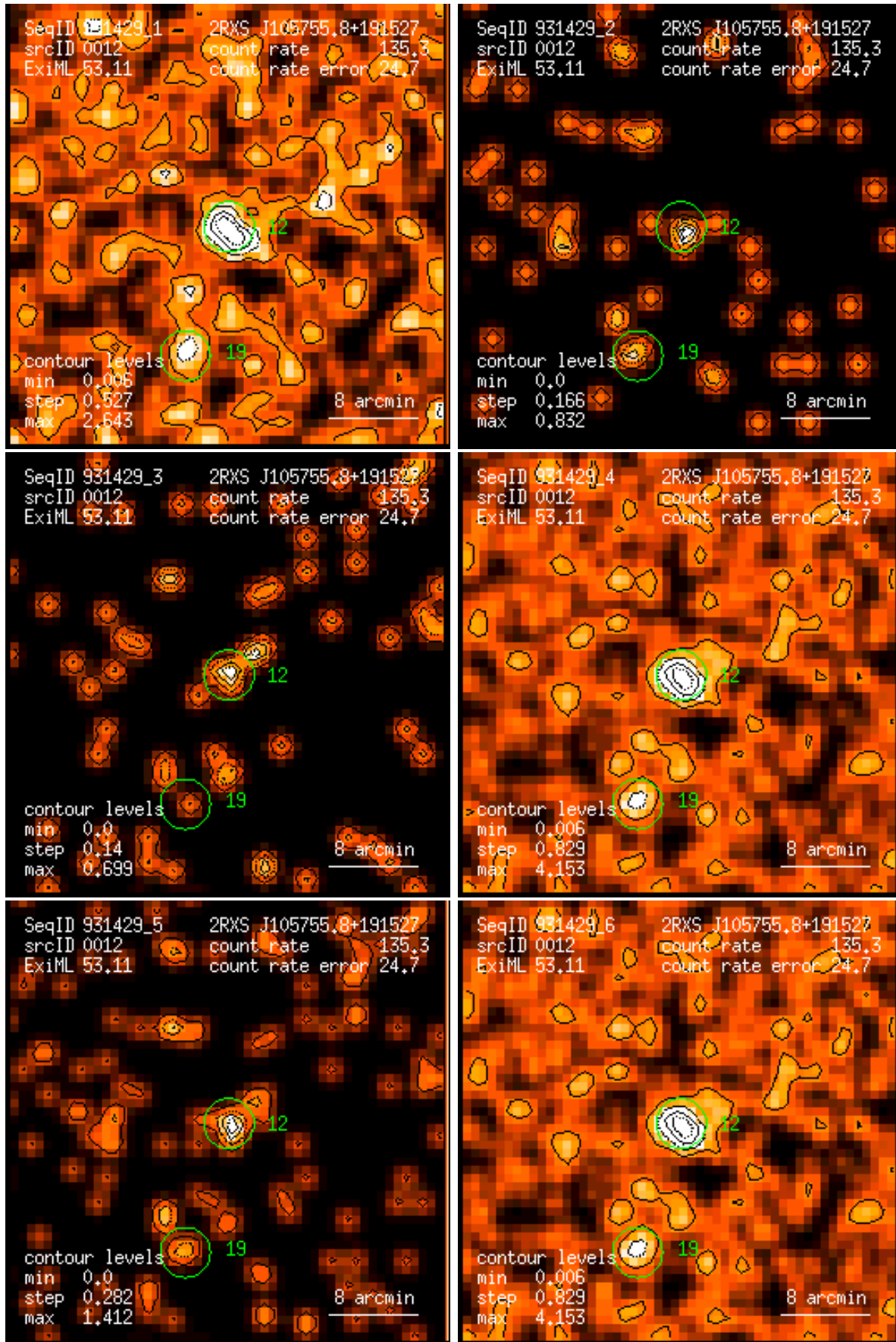
Figure 12: RASS 931429: detection 0012: band rate images, Gaussian filter: (1) PSPC channels 11 – 41, (2) 52 – 90, (3) 91 – 201, (4) 11 – 235, (5) 52 – 201, (6) 11 – 201. Broad band rates in counts/ks. Band rate contour levels in counts/ks/arcmin 2 .
