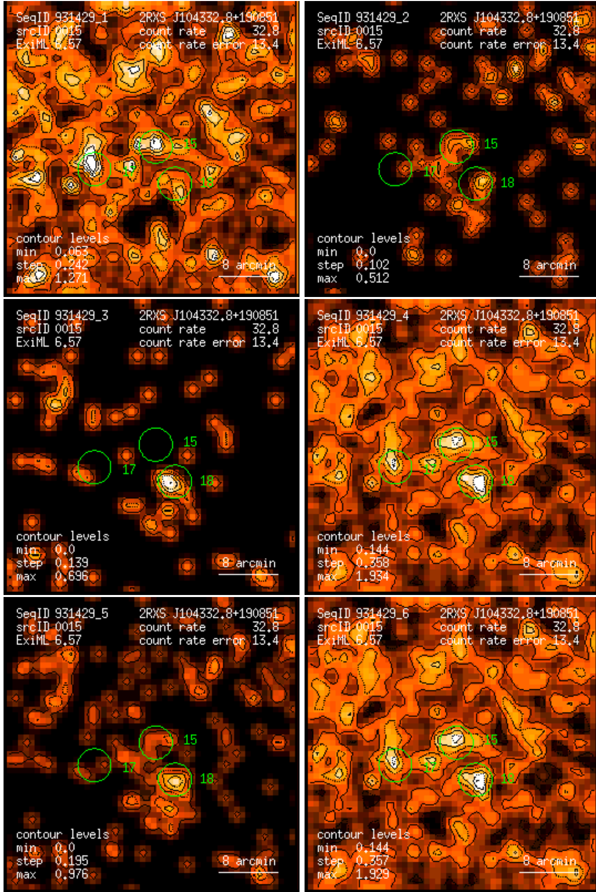
Figure 15: RASS 931429: detection 0015: band rate images, Gaussian filter: (1) PSPC channels 11 – 41, (2) 52 – 90, (3) 91 – 201, (4) 11 – 235, (5) 52 – 201, (6) 11 – 201. Broad band rates in counts/ks. Band rate contour levels in counts/ks/arcmin 2 .
