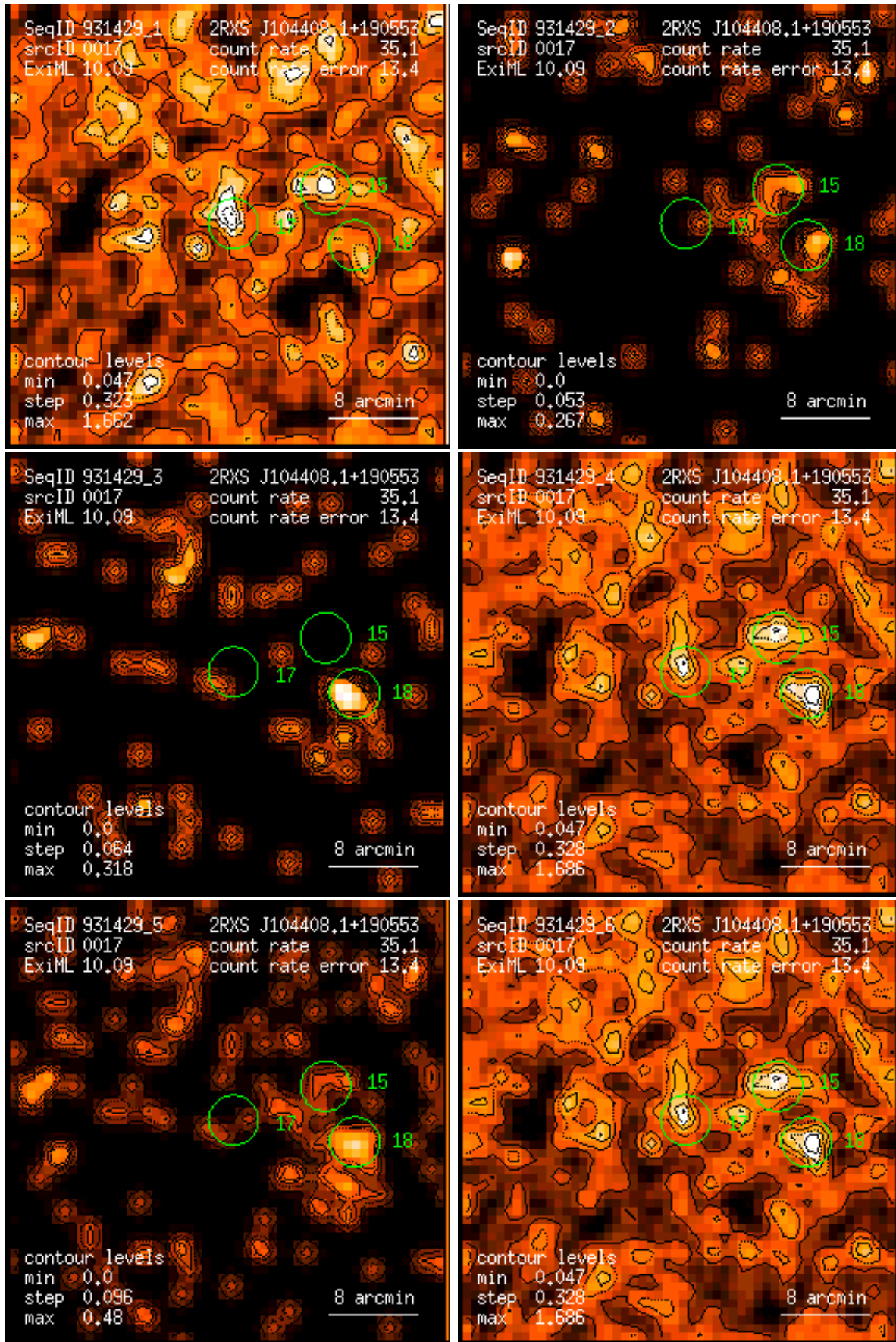
Figure 17: RASS 931429: detection 0017: band rate images, Gaussian filter: (1) PSPC channels 11 – 41, (2) 52 – 90, (3) 91 – 201, (4) 11 – 235, (5) 52 – 201, (6) 11 – 201. Broad band rates in counts/ks. Band rate contour levels in counts/ks/arcmin 2 .
