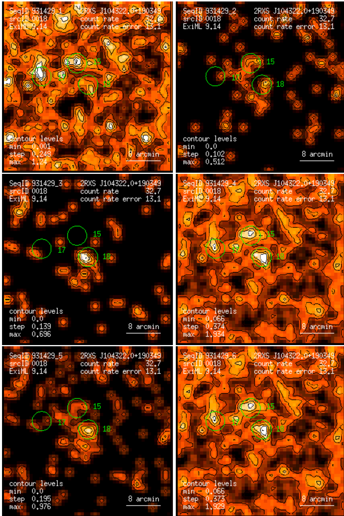
Figure 18: RASS 931429: detection 0018: band rate images, Gaussian filter: (1) PSPC channels 11 – 41, (2) 52 – 90, (3) 91 – 201, (4) 11 – 235, (5) 52 – 201, (6) 11 – 201. Broad band rates in counts/ks. Band rate contour levels in counts/ks/arcmin 2 .
