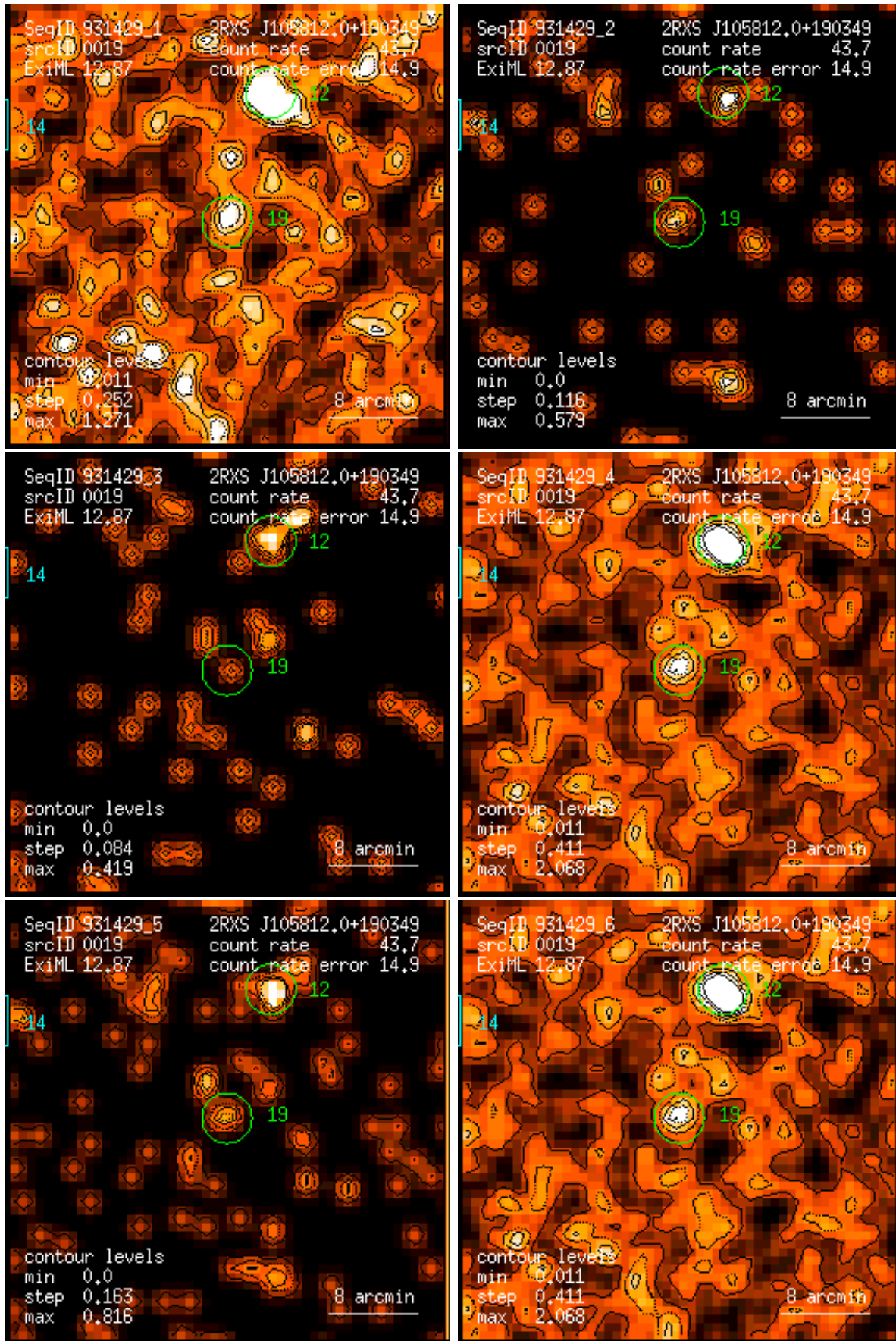
Figure 19: RASS 931429: detection 0019: band rate images, Gaussian filter: (1) PSPC channels 11 – 41, (2) 52 – 90, (3) 91 – 201, (4) 11 – 235, (5) 52 – 201, (6) 11 – 201. Broad band rates in counts/ks. Band rate contour levels in counts/ks/arcmin 2 .
