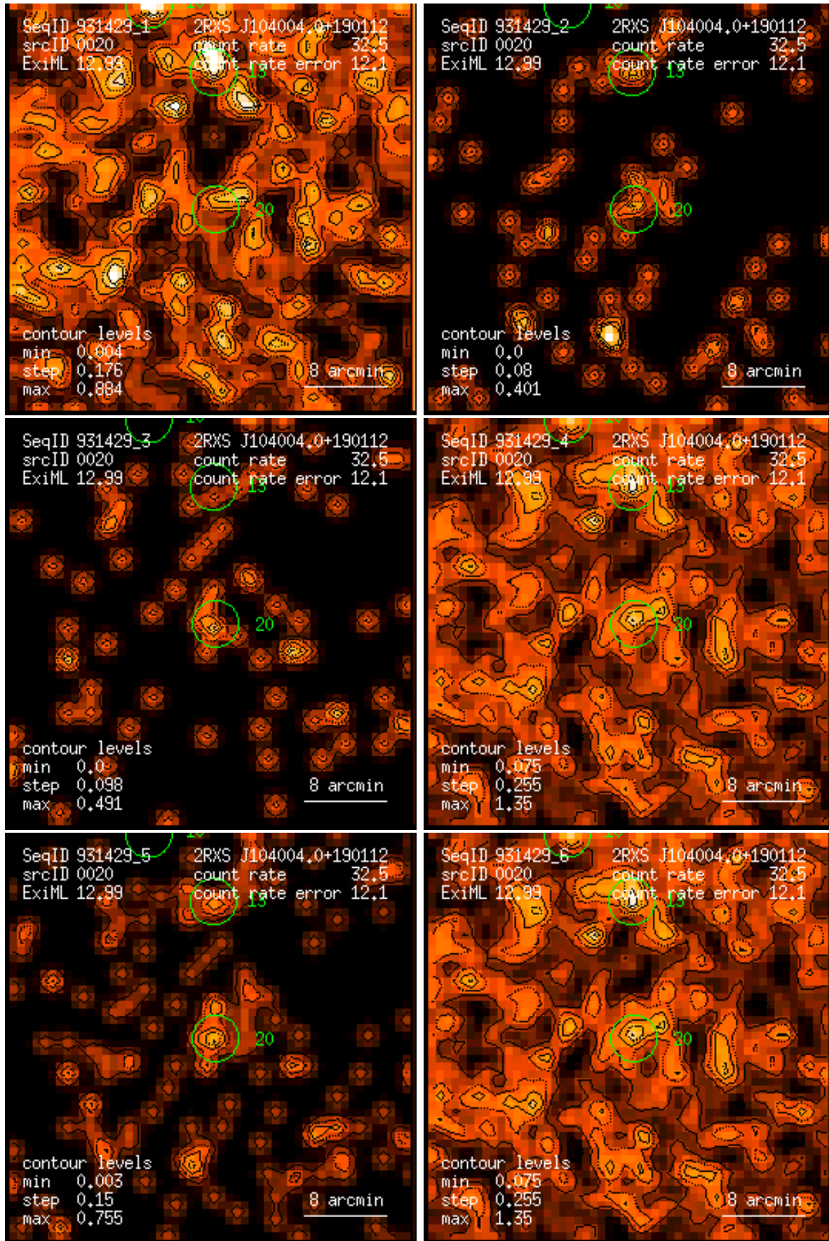
Figure 20: RASS 931429: detection 0020: band rate images, Gaussian filter: (1) PSPC channels 11 – 41, (2) 52 – 90, (3) 91 – 201, (4) 11 – 235, (5) 52 – 201, (6) 11 – 201. Broad band rates in counts/ks. Band rate contour levels in counts/ks/arcmin 2 .
