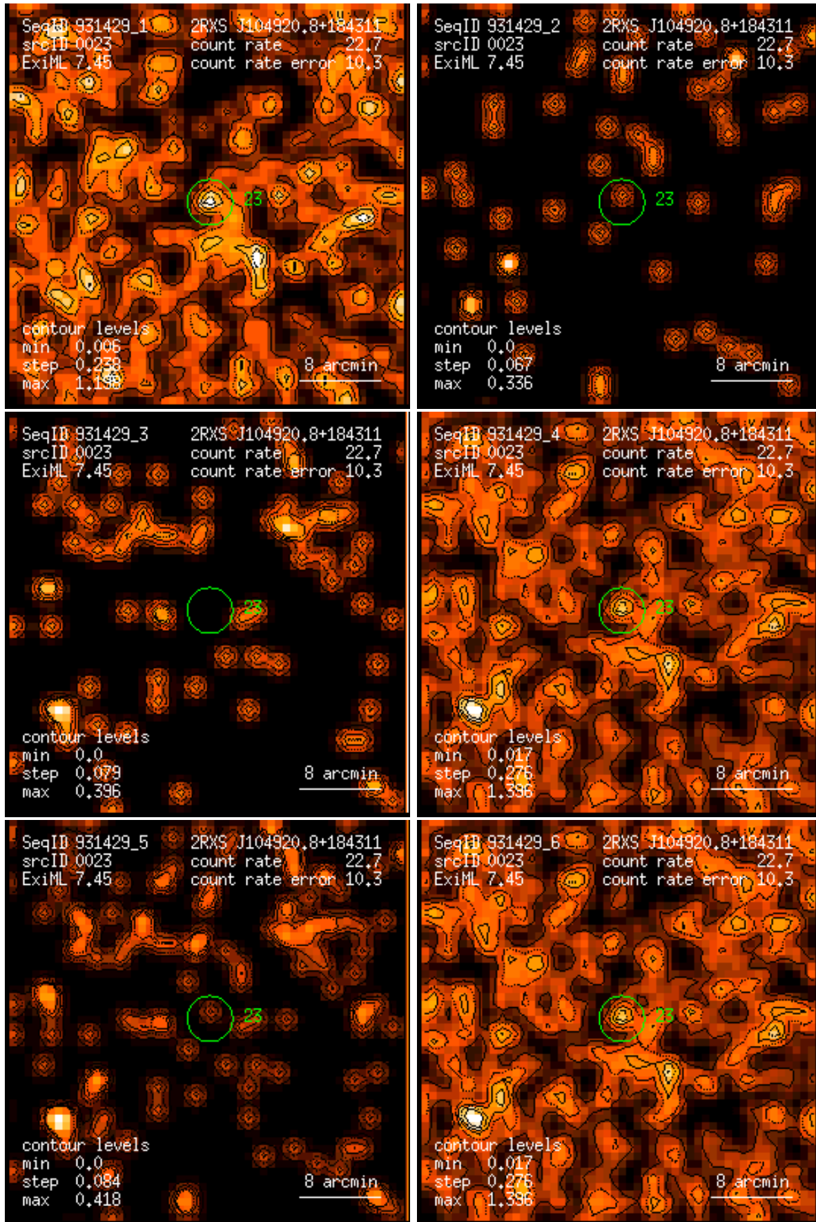
Figure 23: RASS 931429: detection 0023: band rate images, Gaussian filter: (1) PSPC channels 11 – 41, (2) 52 – 90, (3) 91 – 201, (4) 11 – 235, (5) 52 – 201, (6) 11 – 201. Broad band rates in counts/ks. Band rate contour levels in counts/ks/arcmin 2 .
