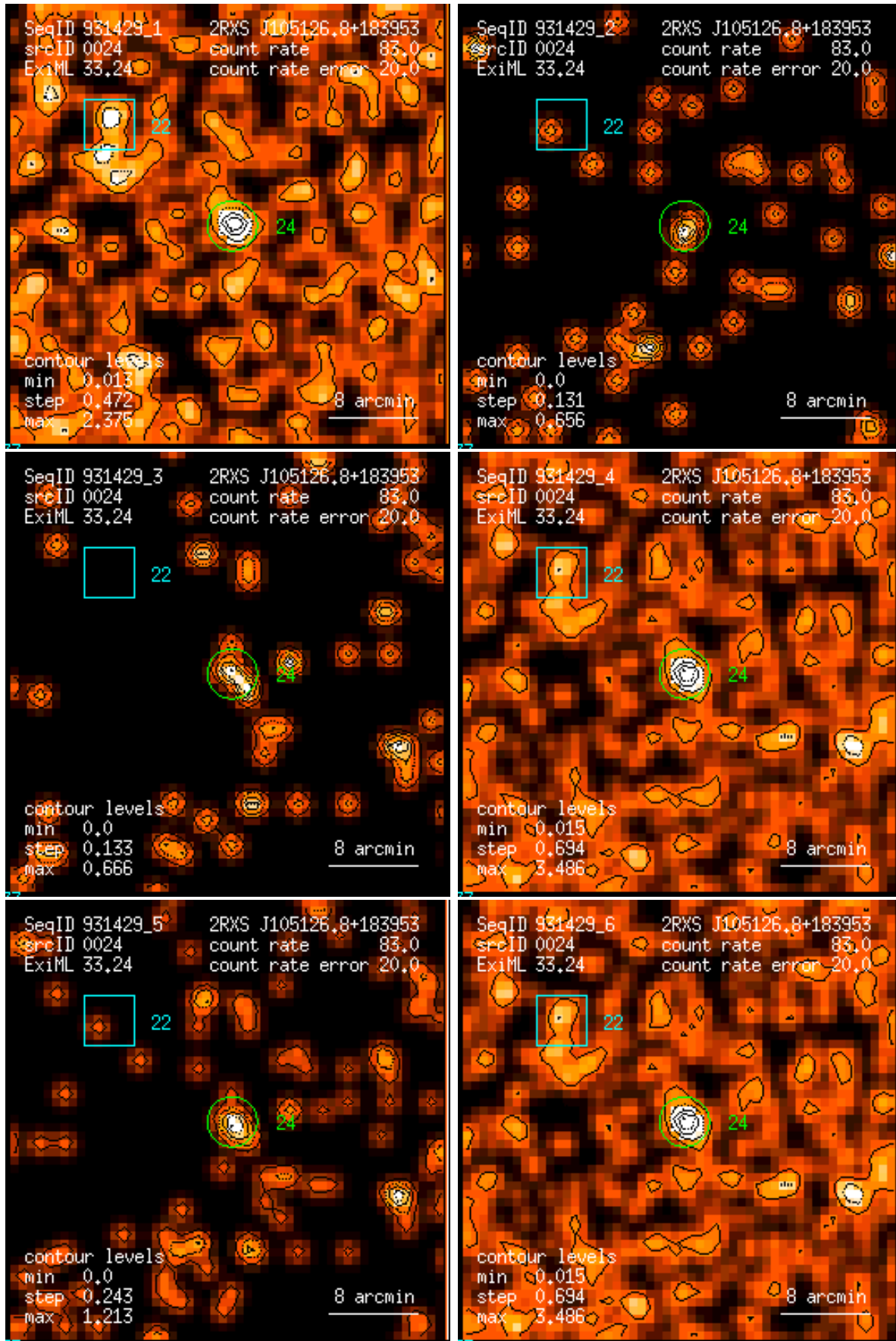
Figure 24: RASS 931429: detection 0024: band rate images, Gaussian filter: (1) PSPC channels 11 – 41, (2) 52 – 90, (3) 91 – 201, (4) 11 – 235, (5) 52 – 201, (6) 11 – 201. Broad band rates in counts/ks. Band rate contour levels in counts/ks/arcmin 2 .
