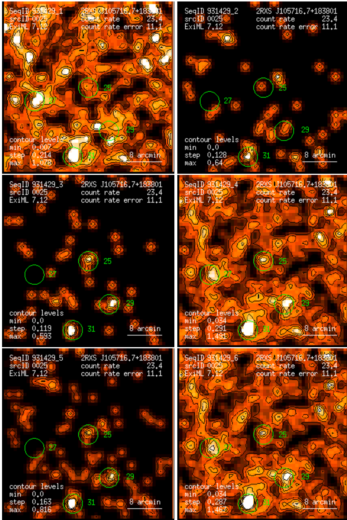
Figure 25: RASS 931429: detection 0025: band rate images, Gaussian filter: (1) PSPC channels 11 – 41, (2) 52 – 90, (3) 91 – 201, (4) 11 – 235, (5) 52 – 201, (6) 11 – 201. Broad band rates in counts/ks. Band rate contour levels in counts/ks/arcmin 2 .
