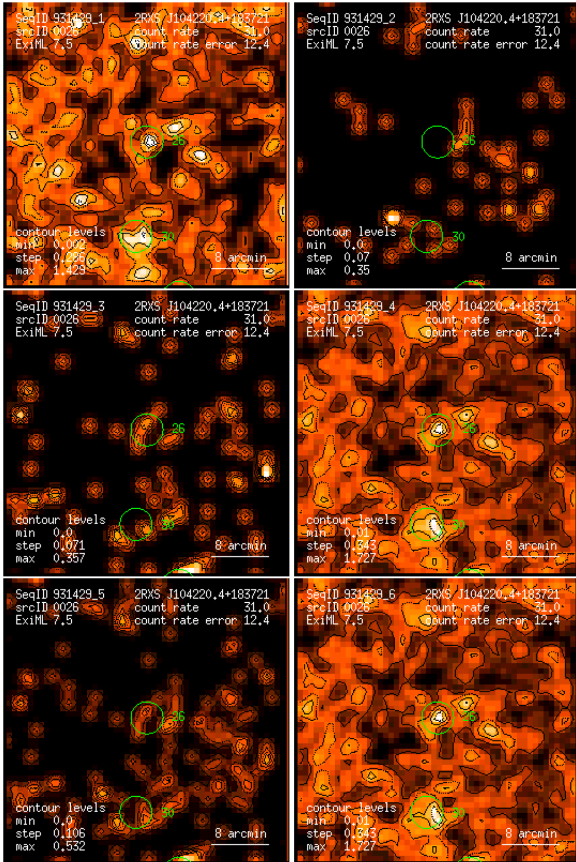
Figure 26: RASS 931429: detection 0026: band rate images, Gaussian filter: (1) PSPC channels 11 – 41, (2) 52 – 90, (3) 91 – 201, (4) 11 – 235, (5) 52 – 201, (6) 11 – 201. Broad band rates in counts/ks. Band rate contour levels in counts/ks/arcmin 2 .
