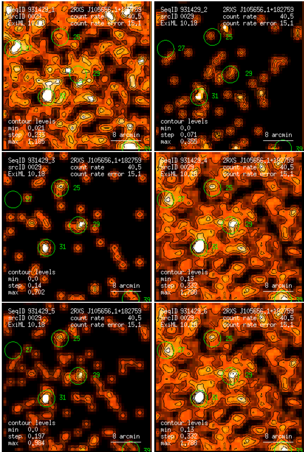
Figure 29: RASS 931429: detection 0029: band rate images, Gaussian filter: (1) PSPC channels 11 – 41, (2) 52 – 90, (3) 91 – 201, (4) 11 – 235, (5) 52 – 201, (6) 11 – 201. Broad band rates in counts/ks. Band rate contour levels in counts/ks/arcmin 2 .
