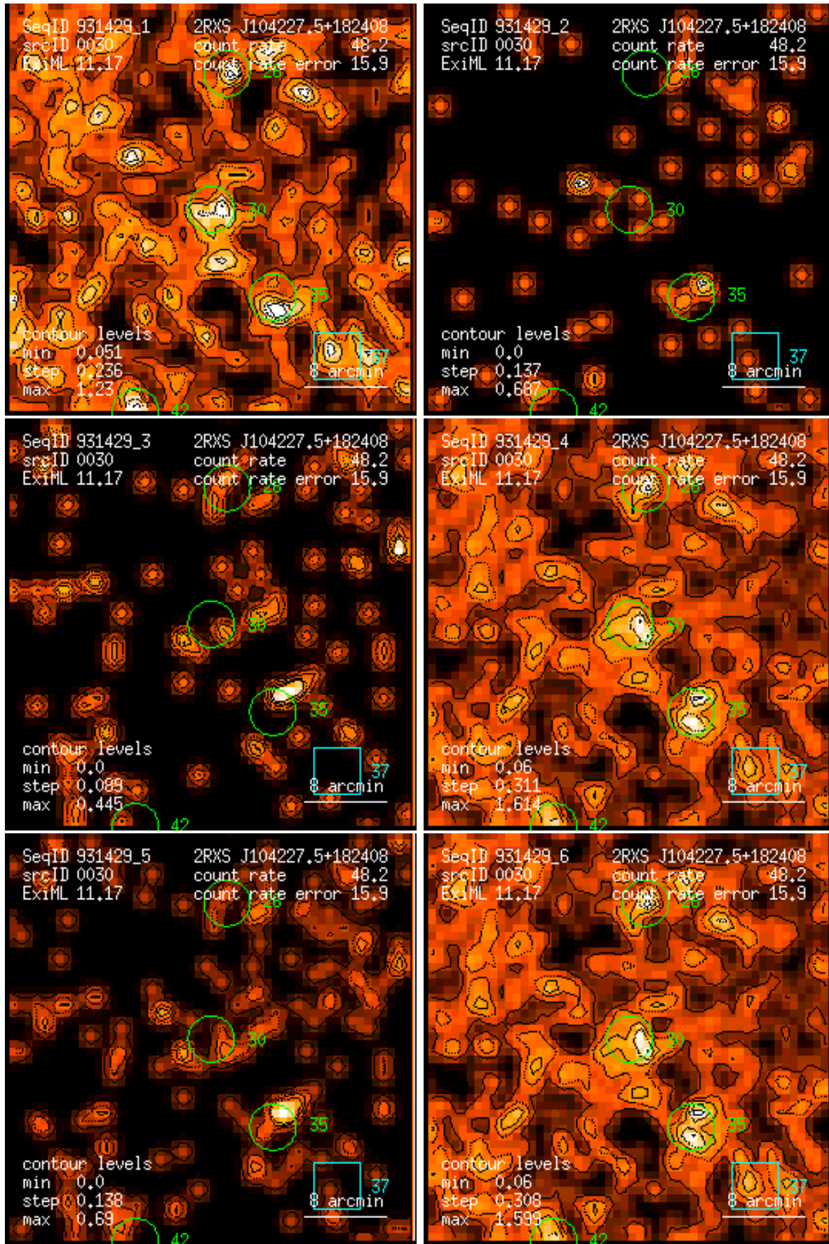
Figure 30: RASS 931429: detection 0030: band rate images, Gaussian filter: (1) PSPC channels 11 – 41, (2) 52 – 90, (3) 91 – 201, (4) 11 – 235, (5) 52 – 201, (6) 11 – 201. Broad band rates in counts/ks. Band rate contour levels in counts/ks/arcmin 2 .
