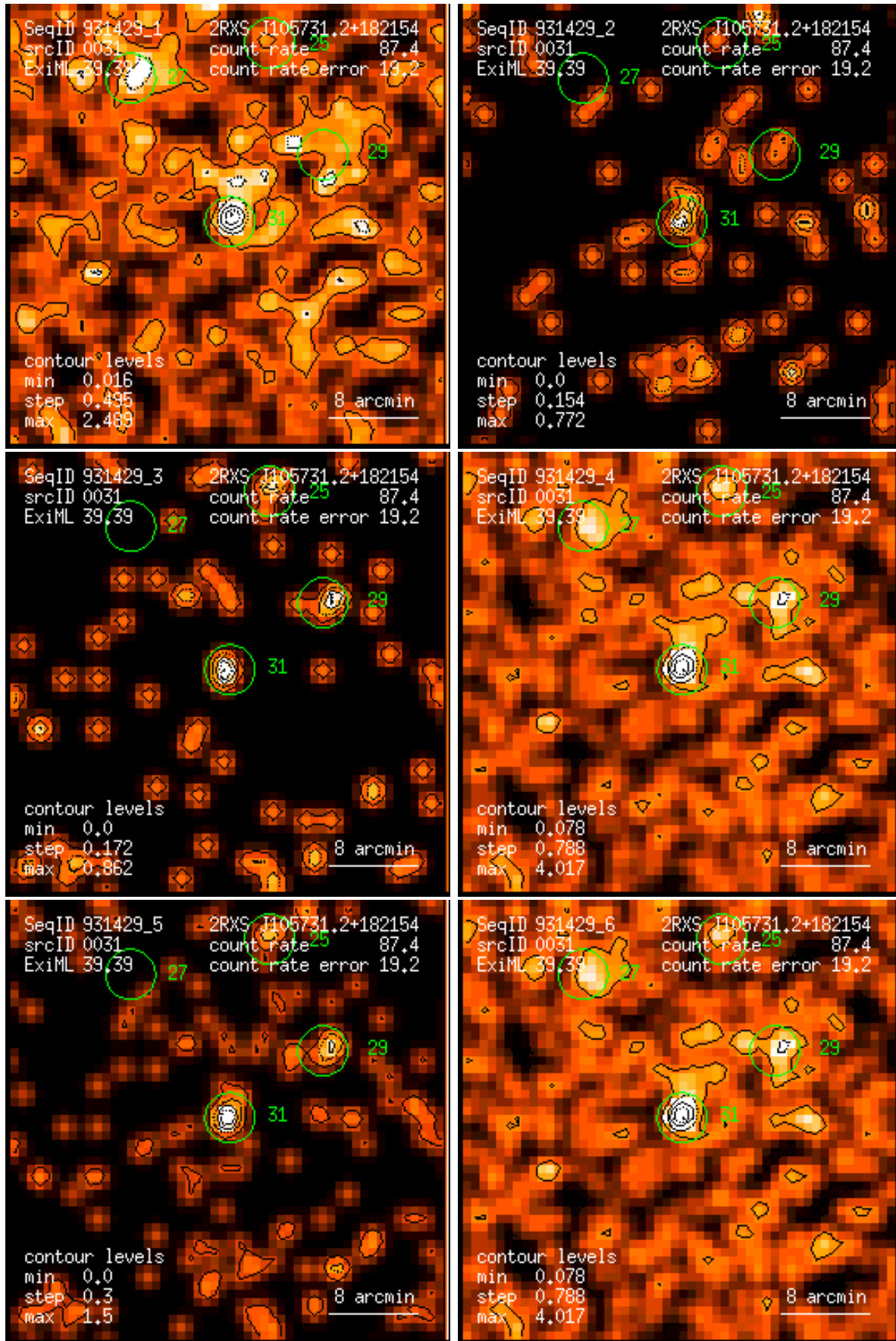
Figure 31: RASS 931429: detection 0031: band rate images, Gaussian filter: (1) PSPC channels 11 – 41, (2) 52 – 90, (3) 91 – 201, (4) 11 – 235, (5) 52 – 201, (6) 11 – 201. Broad band rates in counts/ks. Band rate contour levels in counts/ks/arcmin 2 .
