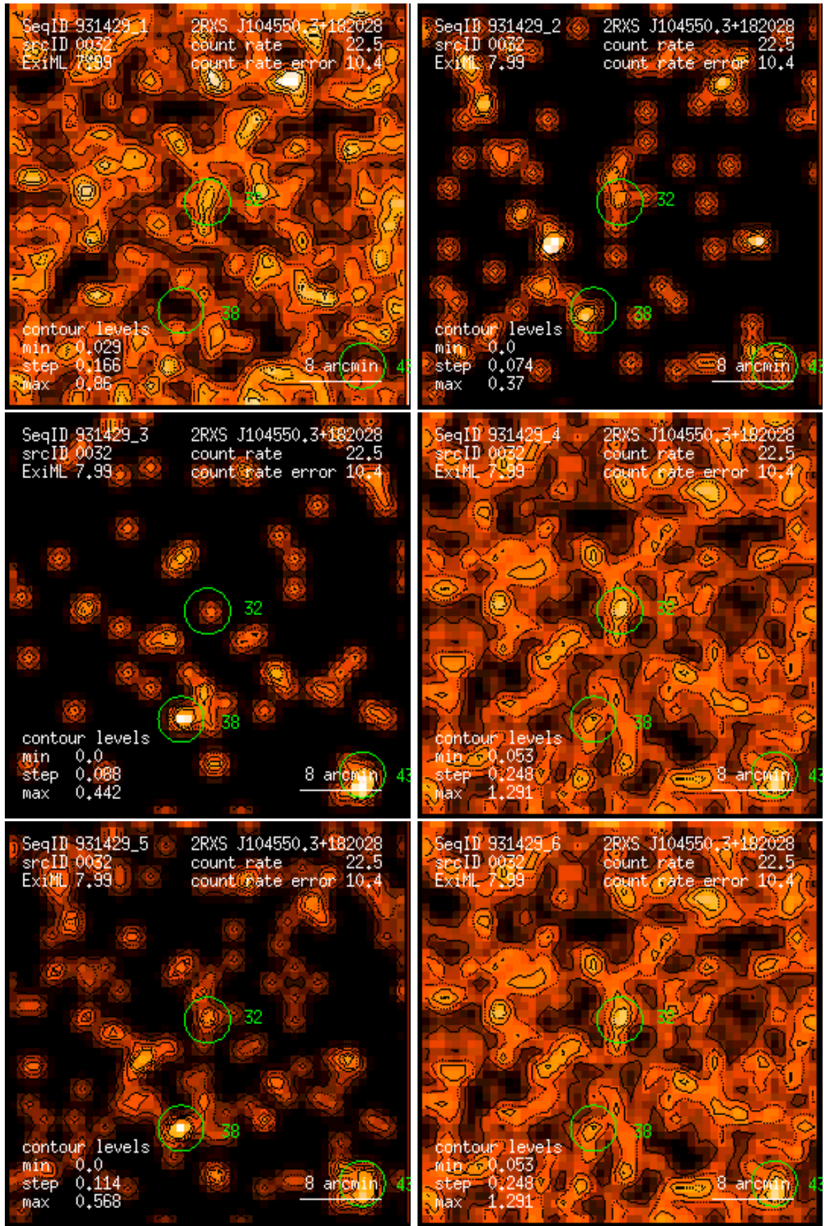
Figure 32: RASS 931429: detection 0032: band rate images, Gaussian filter: (1) PSPC channels 11 – 41, (2) 52 – 90, (3) 91 – 201, (4) 11 – 235, (5) 52 – 201, (6) 11 – 201. Broad band rates in counts/ks. Band rate contour levels in counts/ks/arcmin 2 .
