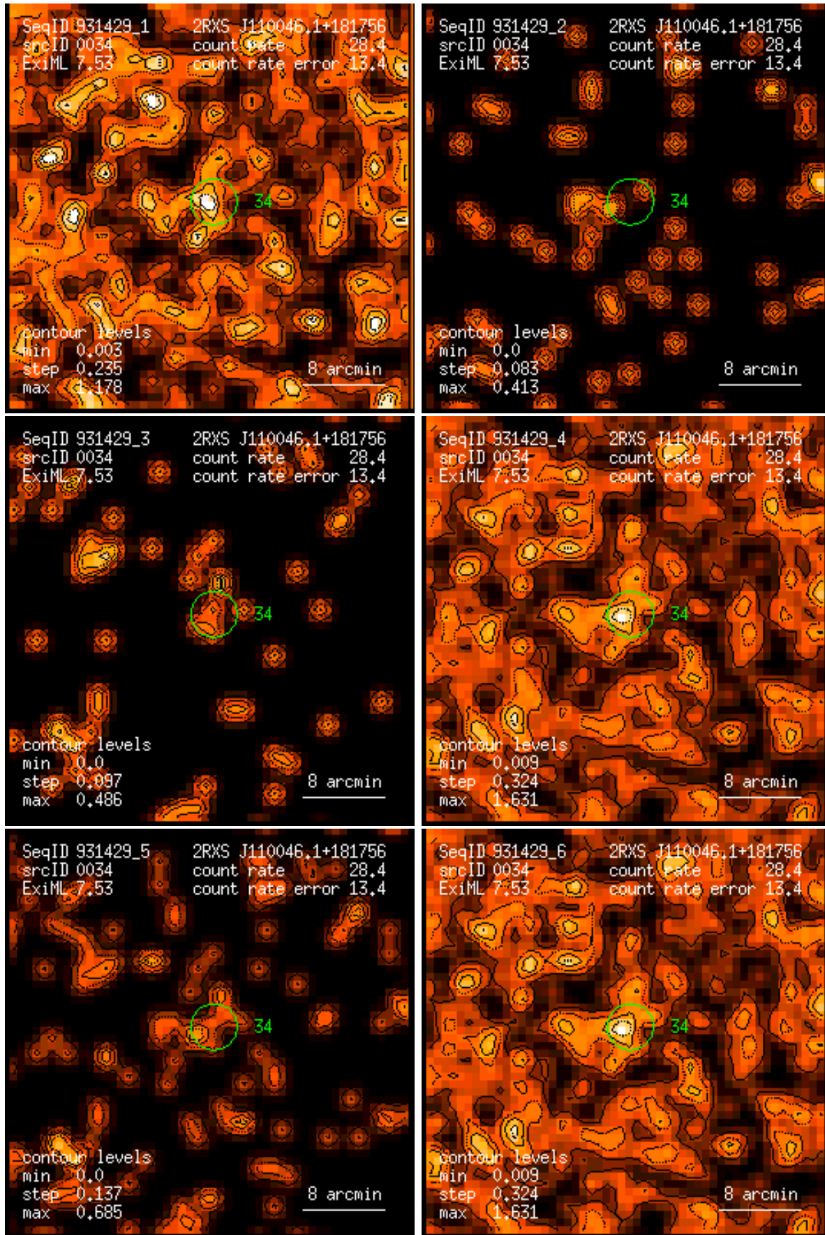
Figure 34: RASS 931429: detection 0034: band rate images, Gaussian filter: (1) PSPC channels 11 – 41, (2) 52 – 90, (3) 91 – 201, (4) 11 – 235, (5) 52 – 201, (6) 11 – 201. Broad band rates in counts/ks. Band rate contour levels in counts/ks/arcmin 2 .
