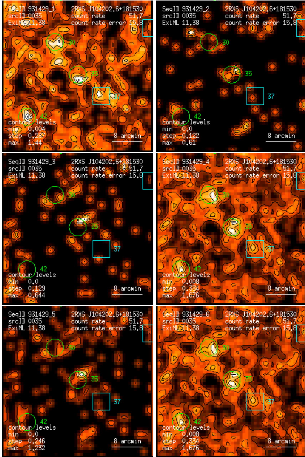
Figure 35: RASS 931429: detection 0035: band rate images, Gaussian filter: (1) PSPC channels 11 – 41, (2) 52 – 90, (3) 91 – 201, (4) 11 – 235, (5) 52 – 201, (6) 11 – 201. Broad band rates in counts/ks. Band rate contour levels in counts/ks/arcmin 2 .
