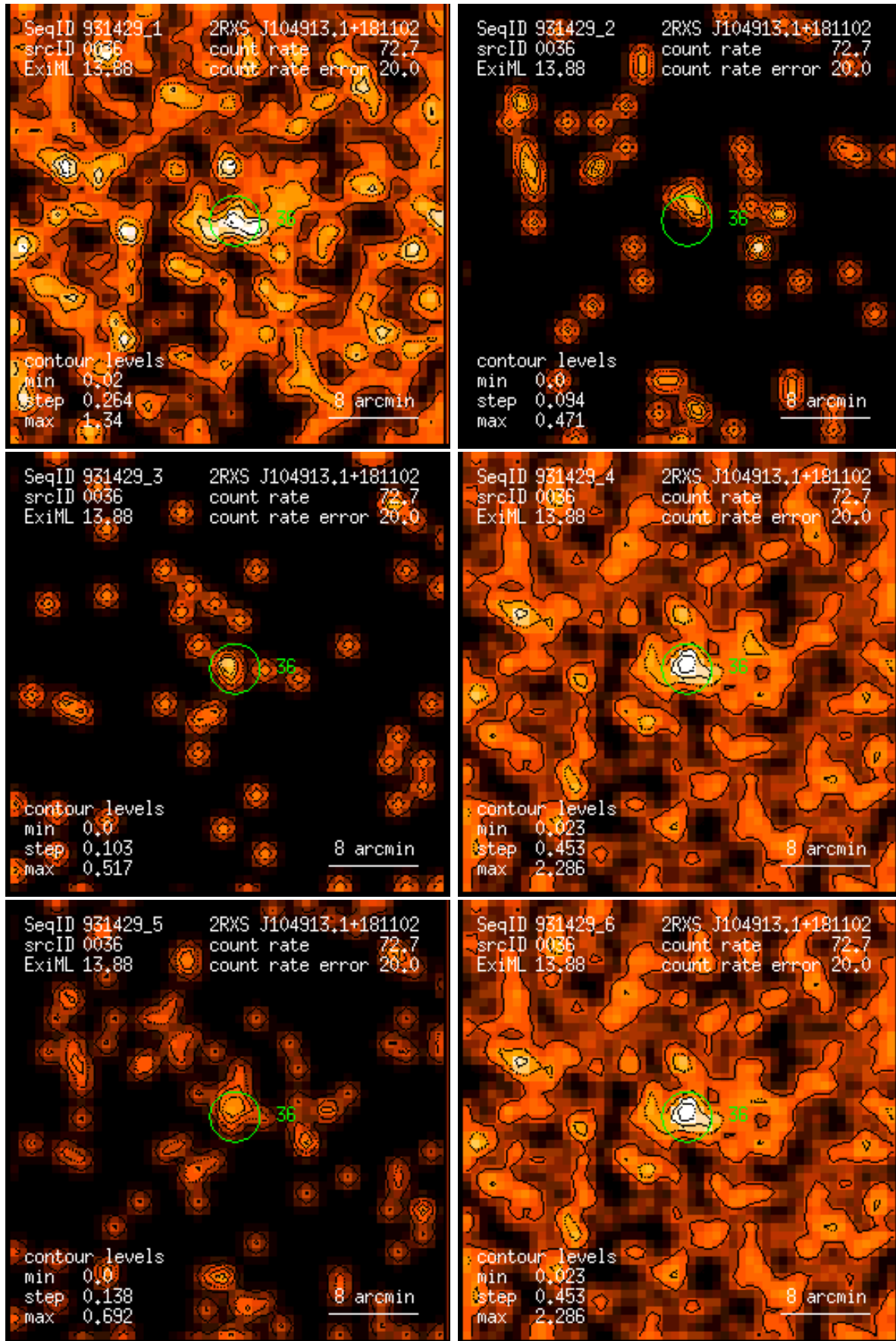
Figure 36: RASS 931429: detection 0036: band rate images, Gaussian filter: (1) PSPC channels 11 – 41, (2) 52 – 90, (3) 91 – 201, (4) 11 – 235, (5) 52 – 201, (6) 11 – 201. Broad band rates in counts/ks. Band rate contour levels in counts/ks/arcmin 2 .
