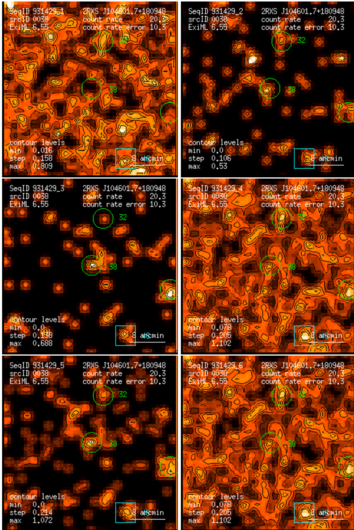
Figure 38: RASS 931429: detection 0038: band rate images, Gaussian filter: (1) PSPC channels 11 – 41, (2) 52 – 90, (3) 91 – 201, (4) 11 – 235, (5) 52 – 201, (6) 11 – 201. Broad band rates in counts/ks. Band rate contour levels in counts/ks/arcmin 2 .
