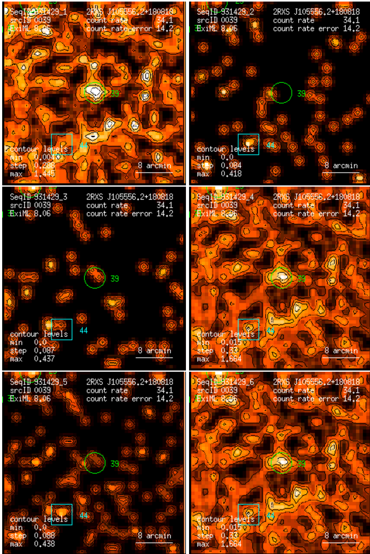
Figure 39: RASS 931429: detection 0039: band rate images, Gaussian filter: (1) PSPC channels 11 – 41, (2) 52 – 90, (3) 91 – 201, (4) 11 – 235, (5) 52 – 201, (6) 11 – 201. Broad band rates in counts/ks. Band rate contour levels in counts/ks/arcmin 2 .
