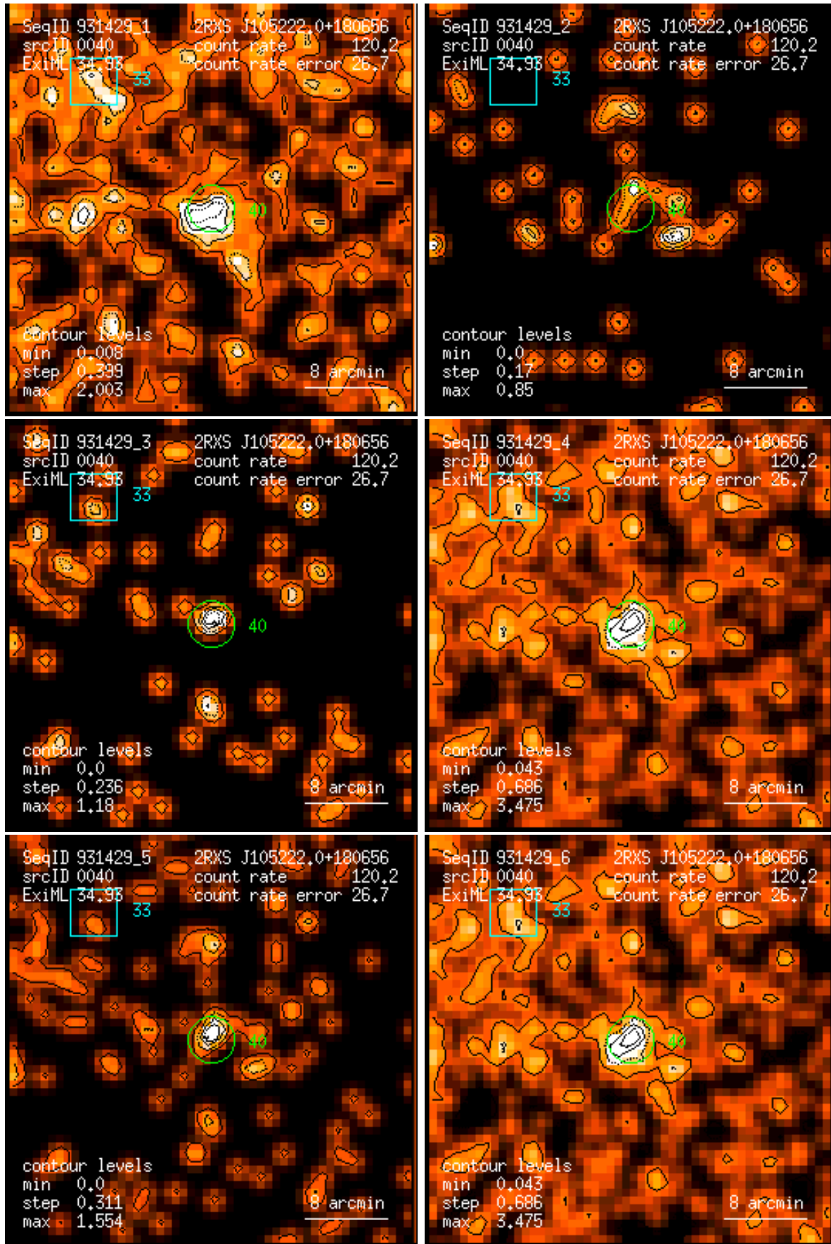
Figure 40: RASS 931429: detection 0040: band rate images, Gaussian filter: (1) PSPC channels 11 – 41, (2) 52 – 90, (3) 91 – 201, (4) 11 – 235, (5) 52 – 201, (6) 11 – 201. Broad band rates in counts/ks. Band rate contour levels in counts/ks/arcmin 2 .
