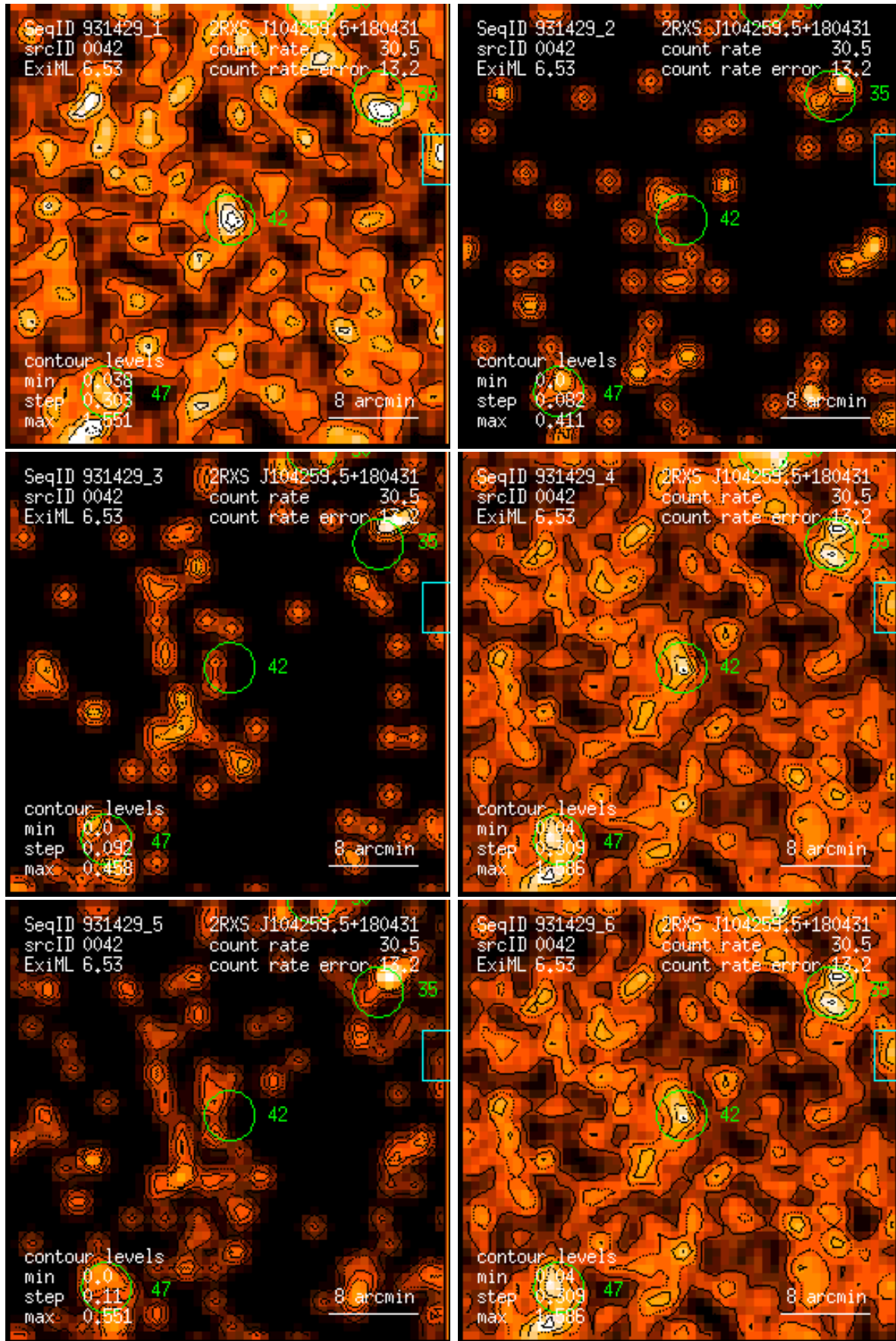
Figure 42: RASS 931429: detection 0042: band rate images, Gaussian filter: (1) PSPC channels 11 – 41, (2) 52 – 90, (3) 91 – 201, (4) 11 – 235, (5) 52 – 201, (6) 11 – 201. Broad band rates in counts/ks. Band rate contour levels in counts/ks/arcmin 2 .
