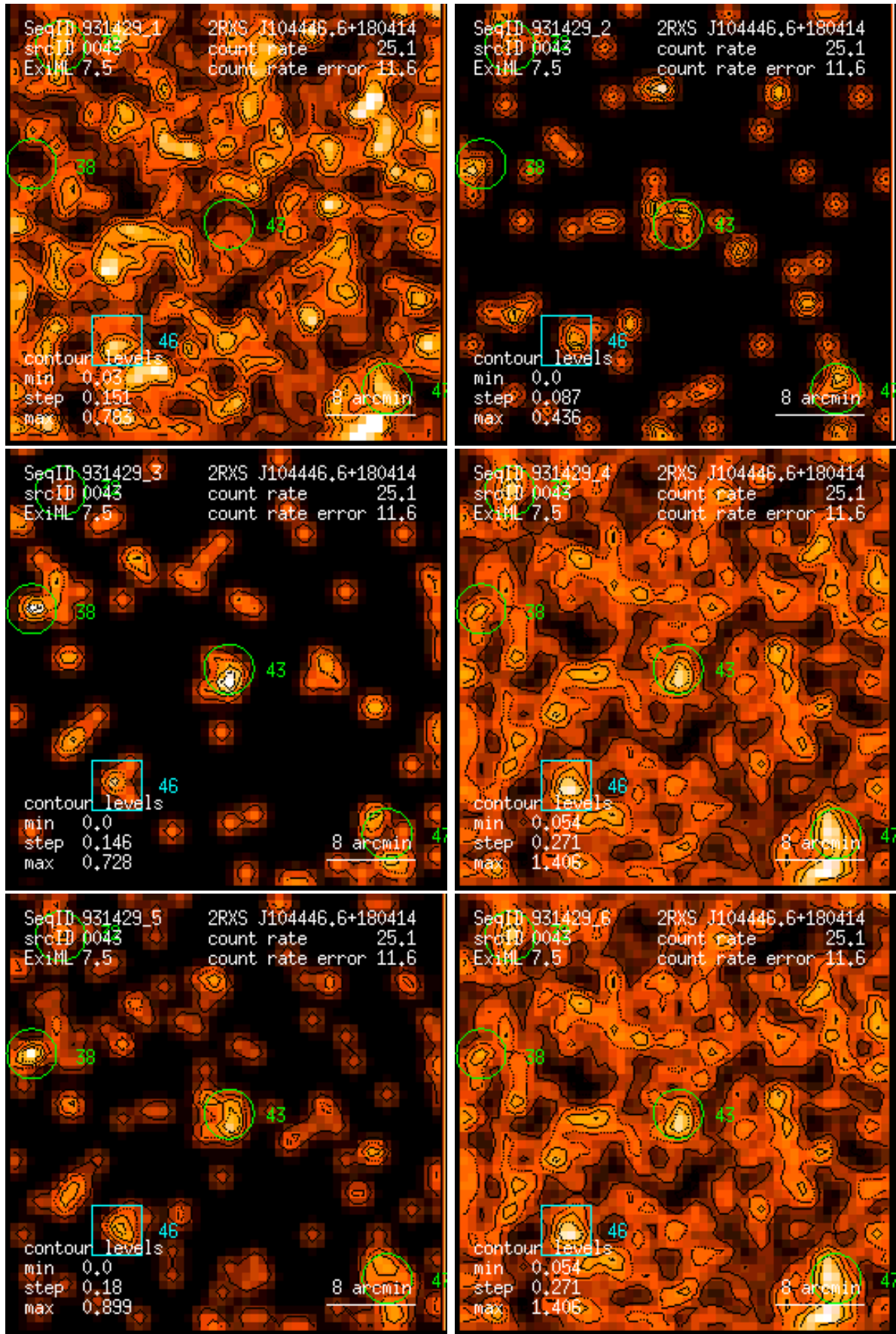
Figure 43: RASS 931429: detection 0043: band rate images, Gaussian filter: (1) PSPC channels 11 – 41, (2) 52 – 90, (3) 91 – 201, (4) 11 – 235, (5) 52 – 201, (6) 11 – 201. Broad band rates in counts/ks. Band rate contour levels in counts/ks/arcmin 2 .
