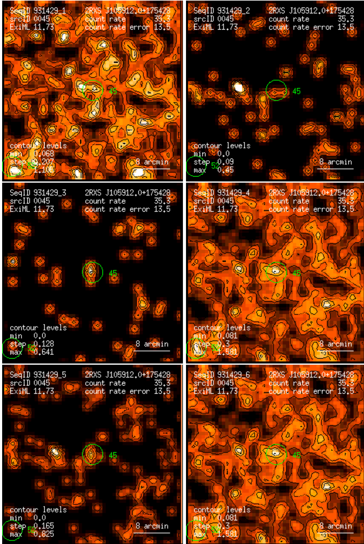
Figure 45: RASS 931429: detection 0045: band rate images, Gaussian filter: (1) PSPC channels 11 – 41, (2) 52 – 90, (3) 91 – 201, (4) 11 – 235, (5) 52 – 201, (6) 11 – 201. Broad band rates in counts/ks. Band rate contour levels in counts/ks/arcmin 2 .
