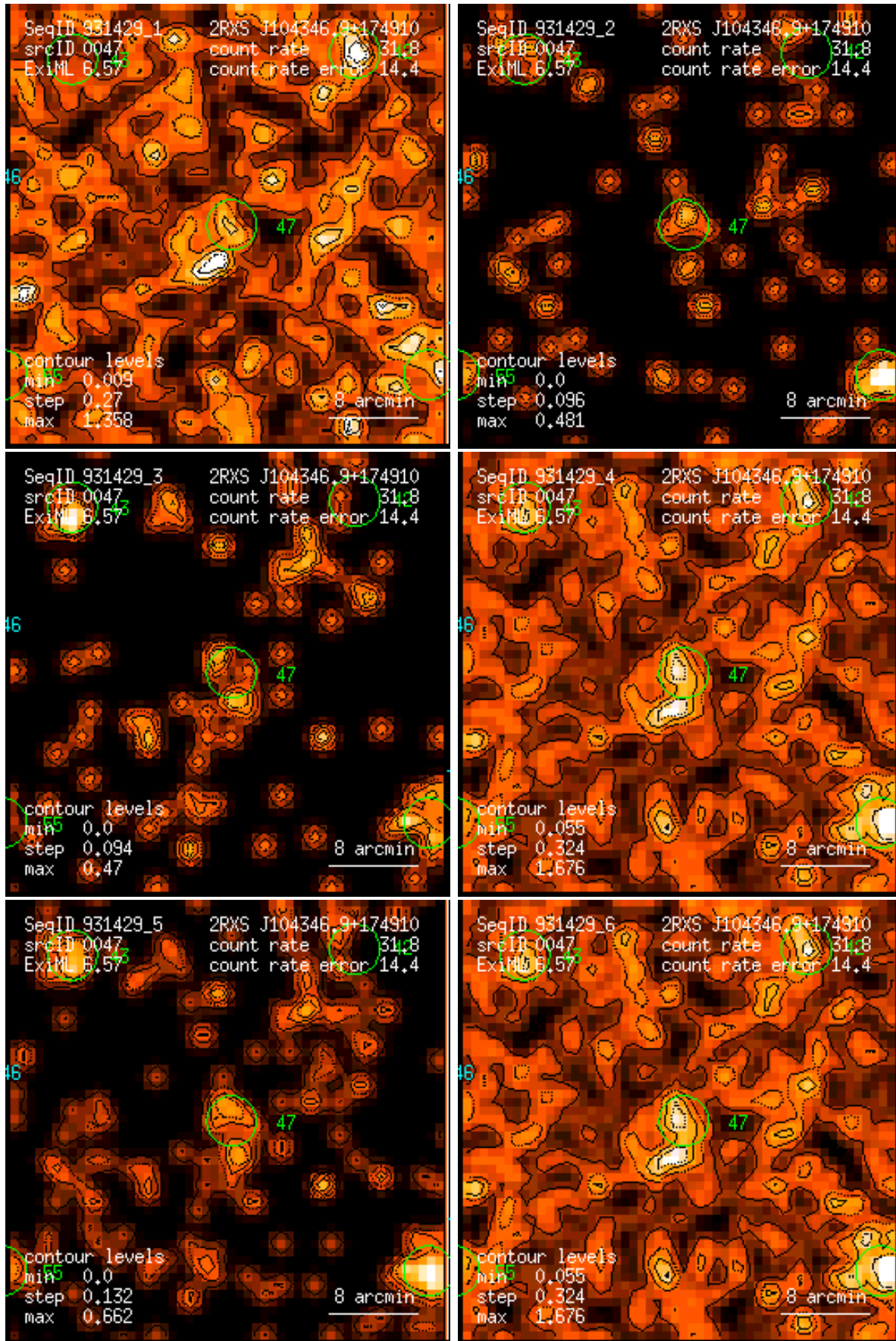
Figure 47: RASS 931429: detection 0047: band rate images, Gaussian filter: (1) PSPC channels 11 – 41, (2) 52 – 90, (3) 91 – 201, (4) 11 – 235, (5) 52 – 201, (6) 11 – 201. Broad band rates in counts/ks. Band rate contour levels in counts/ks/arcmin 2 .
