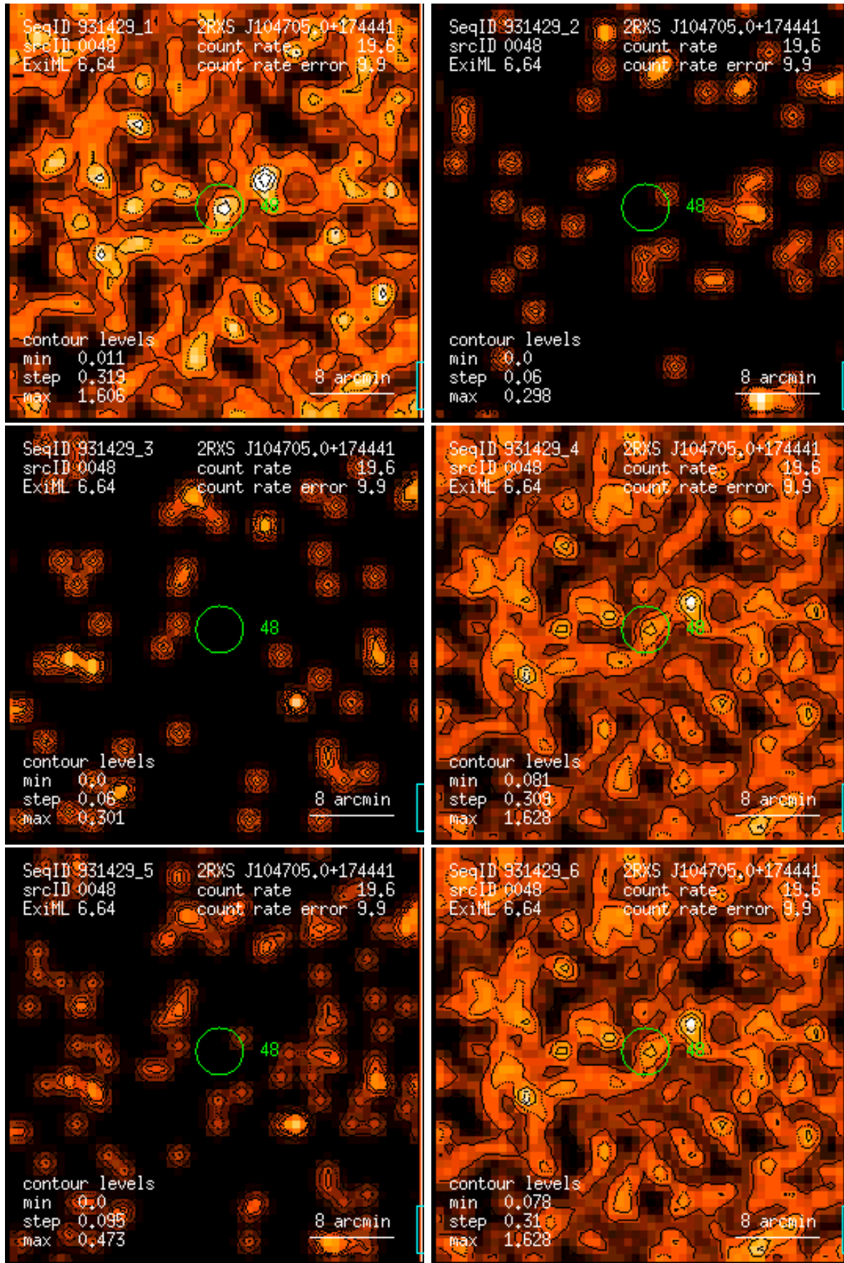
Figure 48: RASS 931429: detection 0048: band rate images, Gaussian filter: (1) PSPC channels 11 – 41, (2) 52 – 90, (3) 91 – 201, (4) 11 – 235, (5) 52 – 201, (6) 11 – 201. Broad band rates in counts/ks. Band rate contour levels in counts/ks/arcmin 2 .
