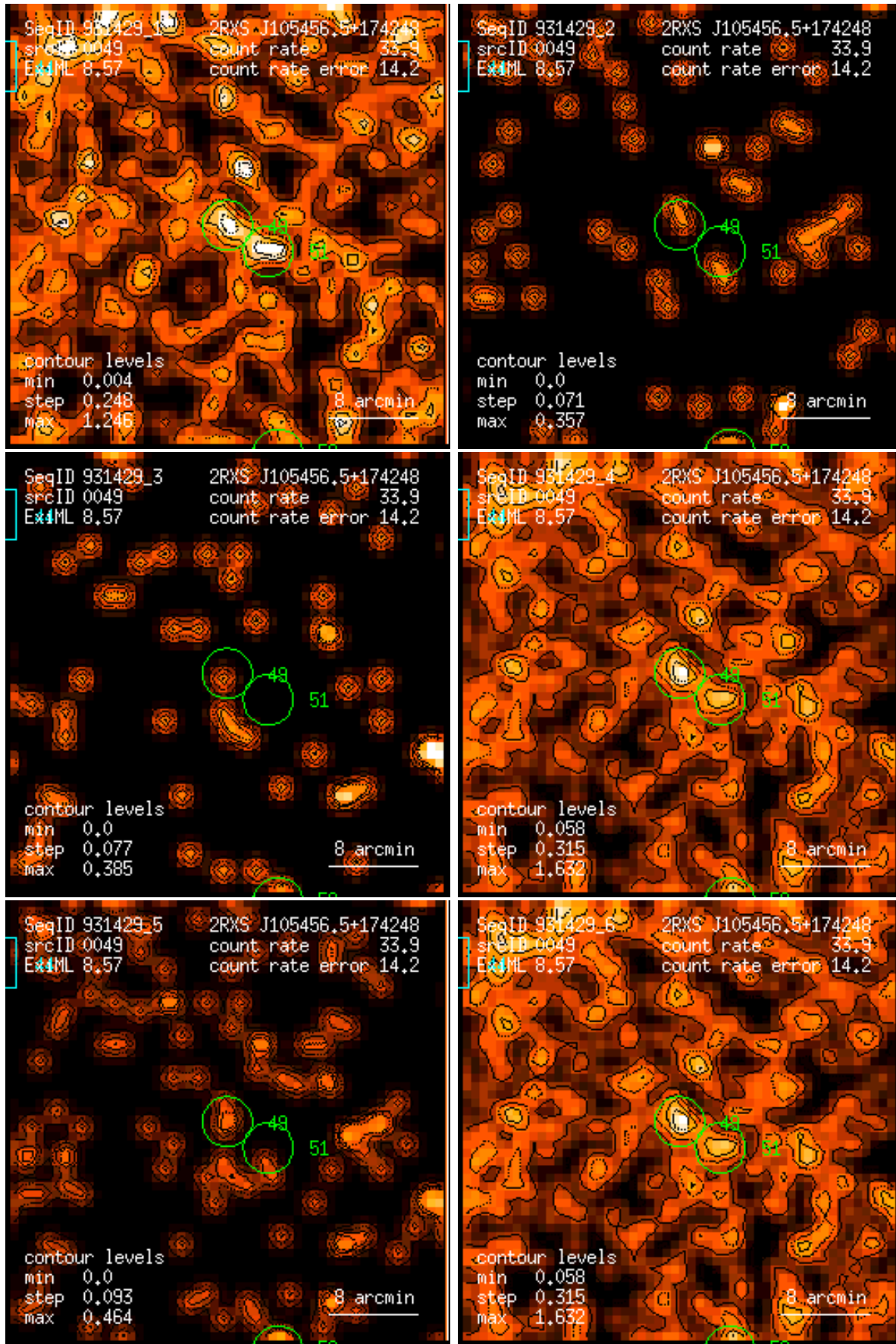
Figure 49: RASS 931429: detection 0049: band rate images, Gaussian filter: (1) PSPC channels 11 – 41, (2) 52 – 90, (3) 91 – 201, (4) 11 – 235, (5) 52 – 201, (6) 11 – 201. Broad band rates in counts/ks. Band rate contour levels in counts/ks/arcmin 2 .
