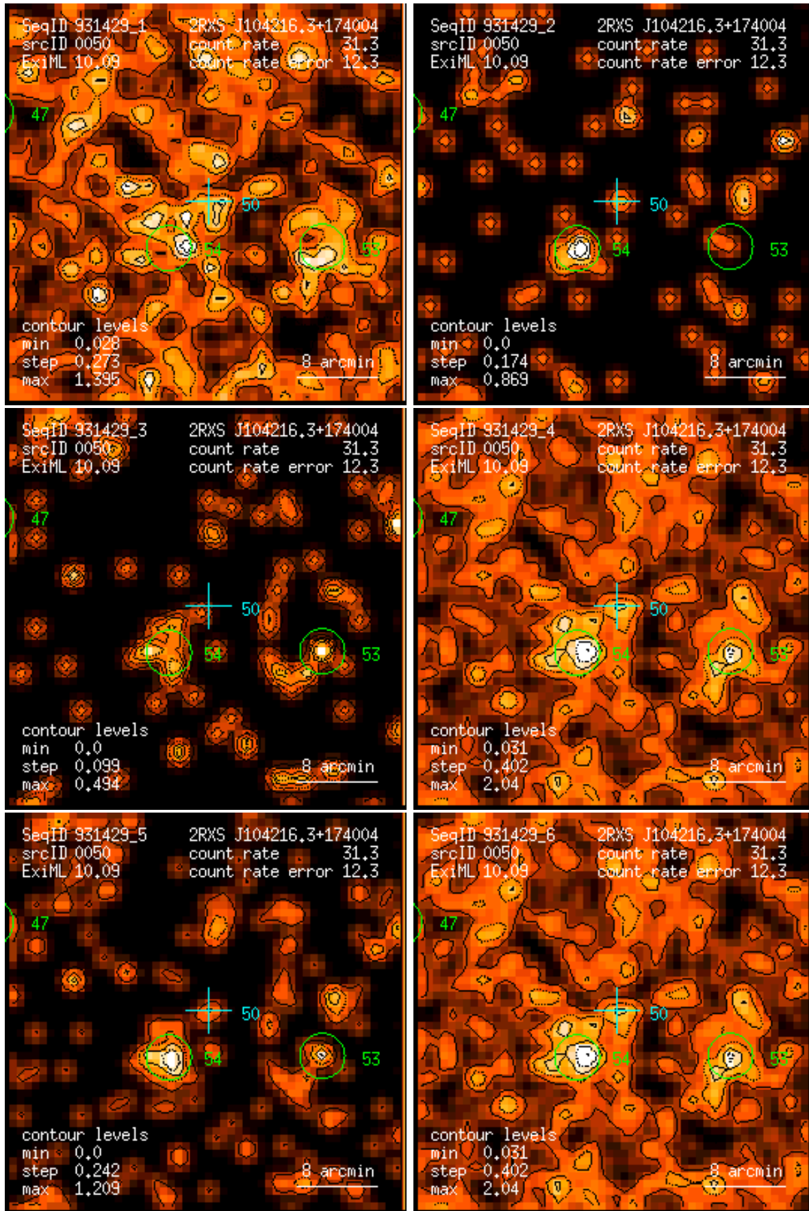
Figure 50: RASS 931429: detection 0050: band rate images, Gaussian filter: (1) PSPC channels 11 – 41, (2) 52 – 90, (3) 91 – 201, (4) 11 – 235, (5) 52 – 201, (6) 11 – 201. Broad band rates in counts/ks. Band rate contour levels in counts/ks/arcmin 2 .
