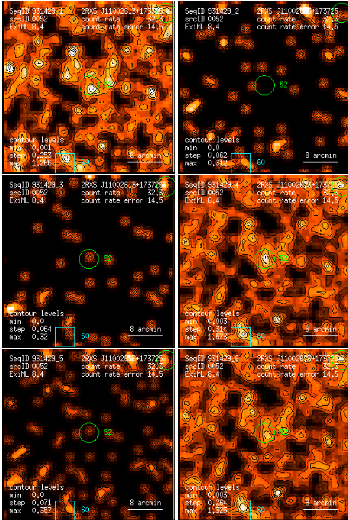
Figure 52: RASS 931429: detection 0052: band rate images, Gaussian filter: (1) PSPC channels 11 – 41, (2) 52 – 90, (3) 91 – 201, (4) 11 – 235, (5) 52 – 201, (6) 11 – 201. Broad band rates in counts/ks. Band rate contour levels in counts/ks/arcmin 2 .
