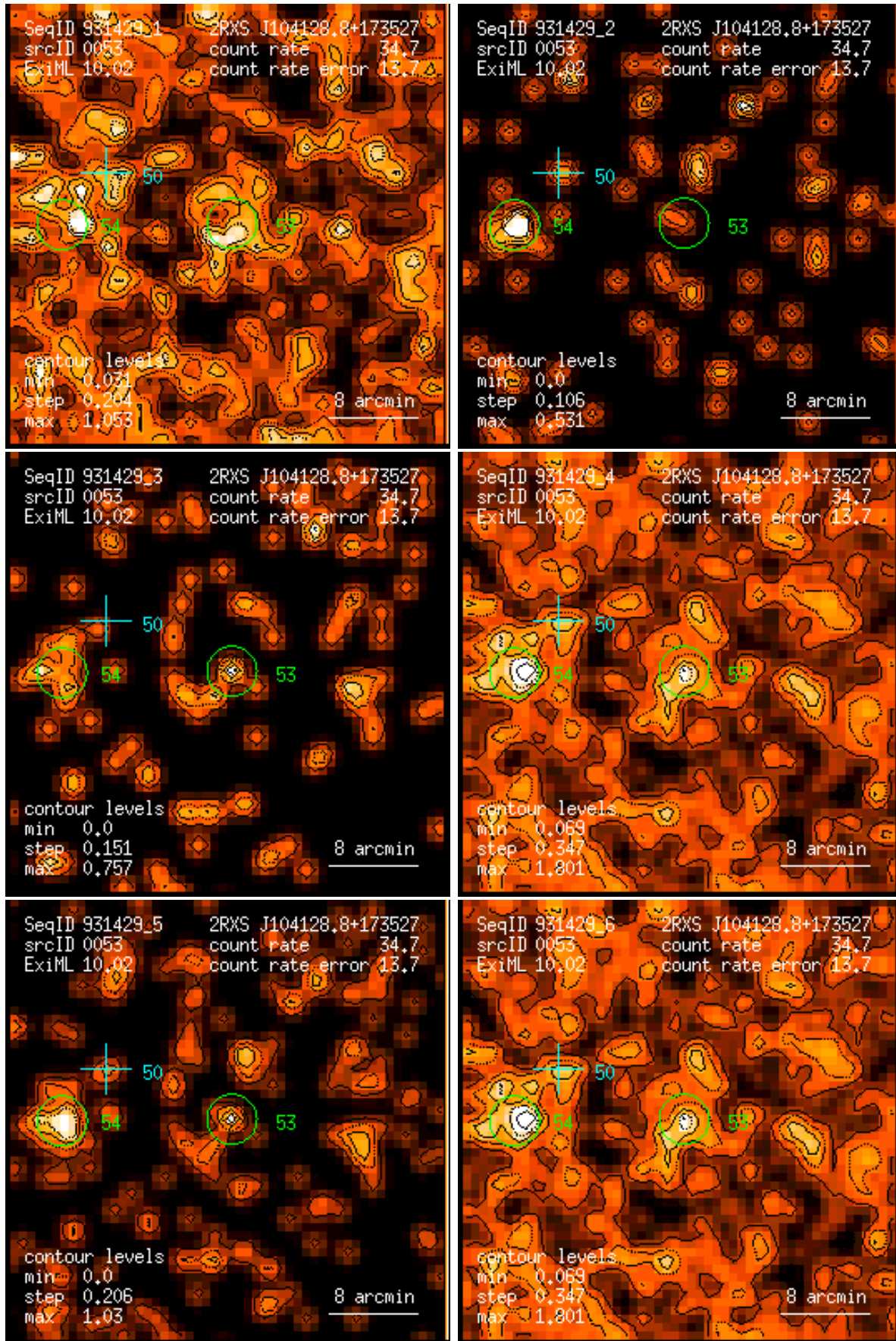
Figure 53: RASS 931429: detection 0053: band rate images, Gaussian filter: (1) PSPC channels 11 – 41, (2) 52 – 90, (3) 91 – 201, (4) 11 – 235, (5) 52 – 201, (6) 11 – 201. Broad band rates in counts/ks. Band rate contour levels in counts/ks/arcmin 2 .
