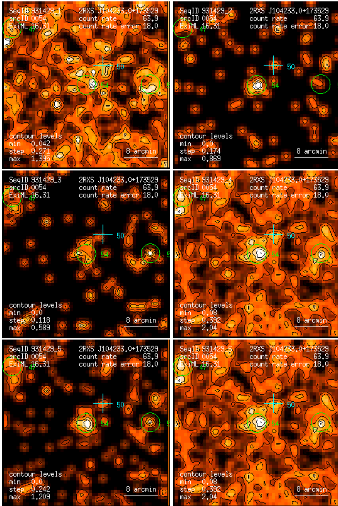
Figure 54: RASS 931429: detection 0054: band rate images, Gaussian filter: (1) PSPC channels 11 – 41, (2) 52 – 90, (3) 91 – 201, (4) 11 – 235, (5) 52 – 201, (6) 11 – 201. Broad band rates in counts/ks. Band rate contour levels in counts/ks/arcmin 2 .
