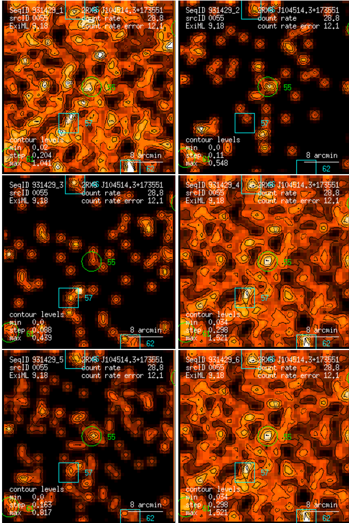
Figure 55: RASS 931429: detection 0055: band rate images, Gaussian filter: (1) PSPC channels 11 – 41, (2) 52 – 90, (3) 91 – 201, (4) 11 – 235, (5) 52 – 201, (6) 11 – 201. Broad band rates in counts/ks. Band rate contour levels in counts/ks/arcmin 2 .
