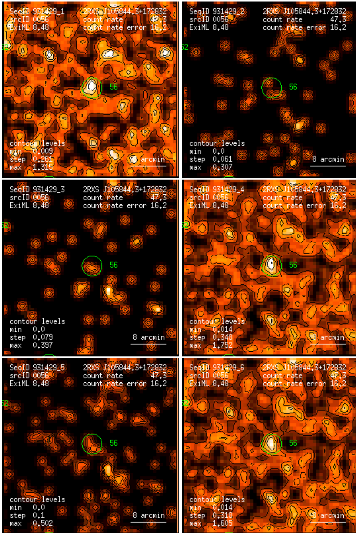
Figure 56: RASS 931429: detection 0056: band rate images, Gaussian filter: (1) PSPC channels 11 – 41, (2) 52 – 90, (3) 91 – 201, (4) 11 – 235, (5) 52 – 201, (6) 11 – 201. Broad band rates in counts/ks. Band rate contour levels in counts/ks/arcmin 2 .
