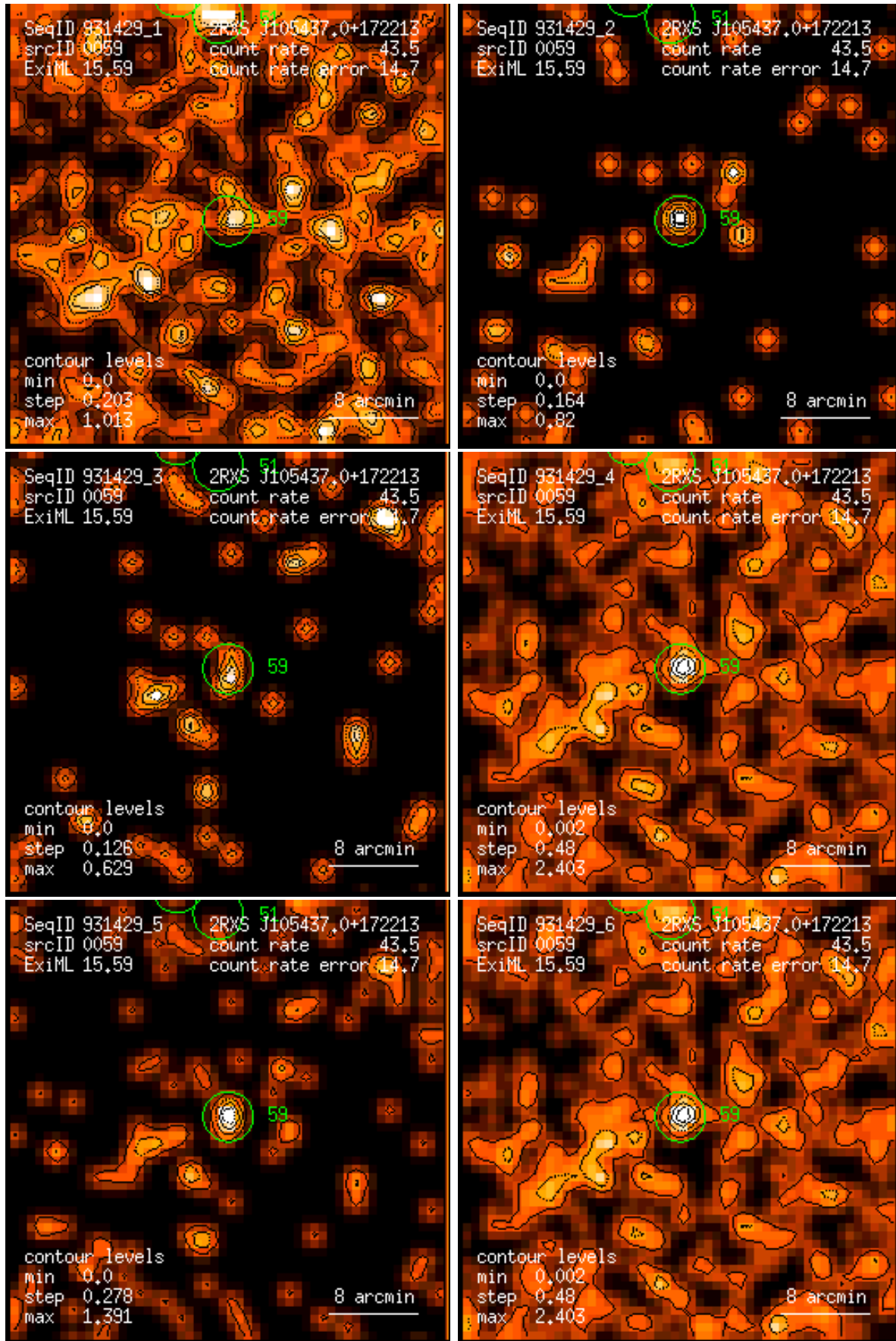
Figure 59: RASS 931429: detection 0059: band rate images, Gaussian filter: (1) PSPC channels 11 – 41, (2) 52 – 90, (3) 91 – 201, (4) 11 – 235, (5) 52 – 201, (6) 11 – 201. Broad band rates in counts/ks. Band rate contour levels in counts/ks/arcmin 2 .
