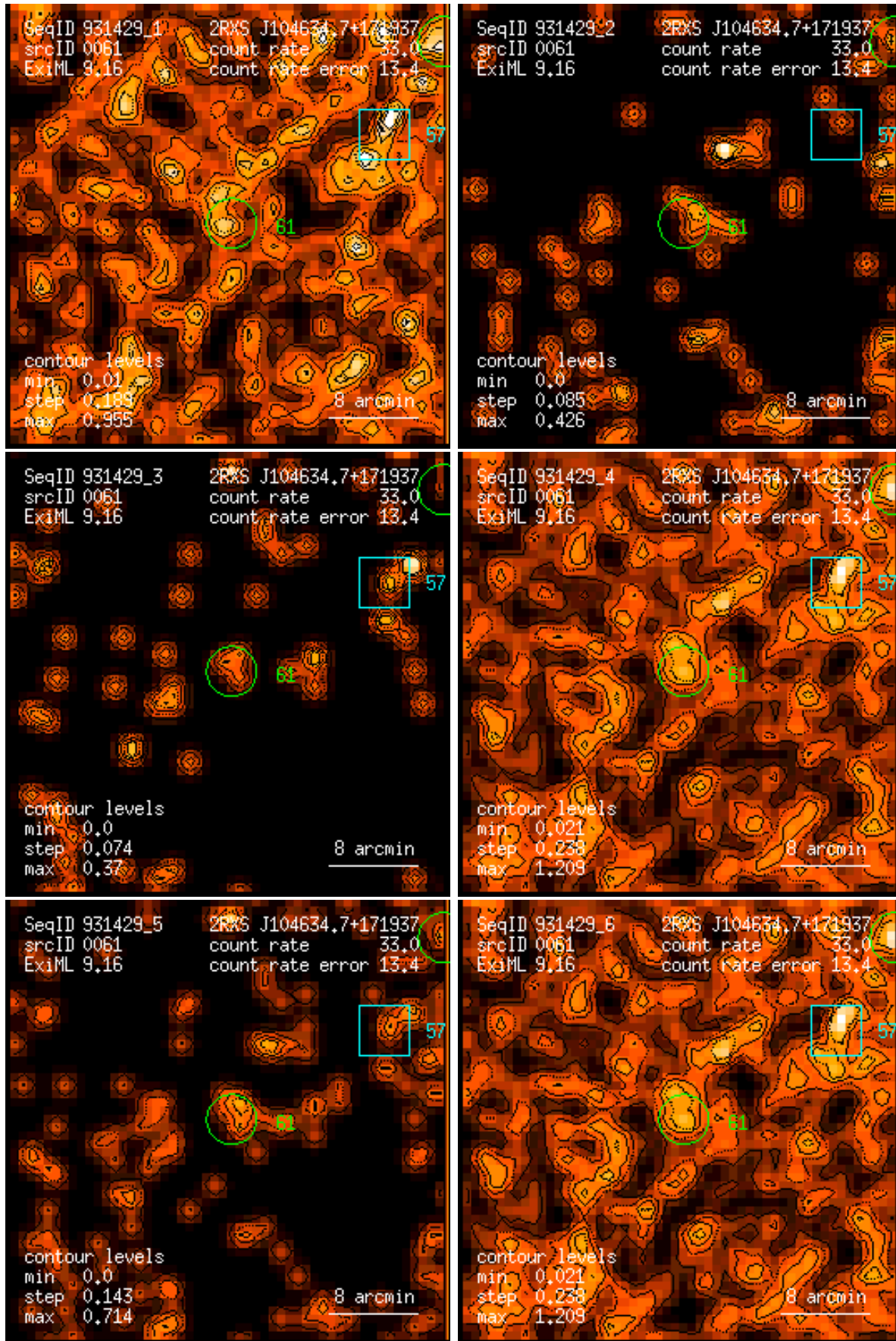
Figure 61: RASS 931429: detection 0061: band rate images, Gaussian filter: (1) PSPC channels 11 – 41, (2) 52 – 90, (3) 91 – 201, (4) 11 – 235, (5) 52 – 201, (6) 11 – 201. Broad band rates in counts/ks. Band rate contour levels in counts/ks/arcmin 2 .
