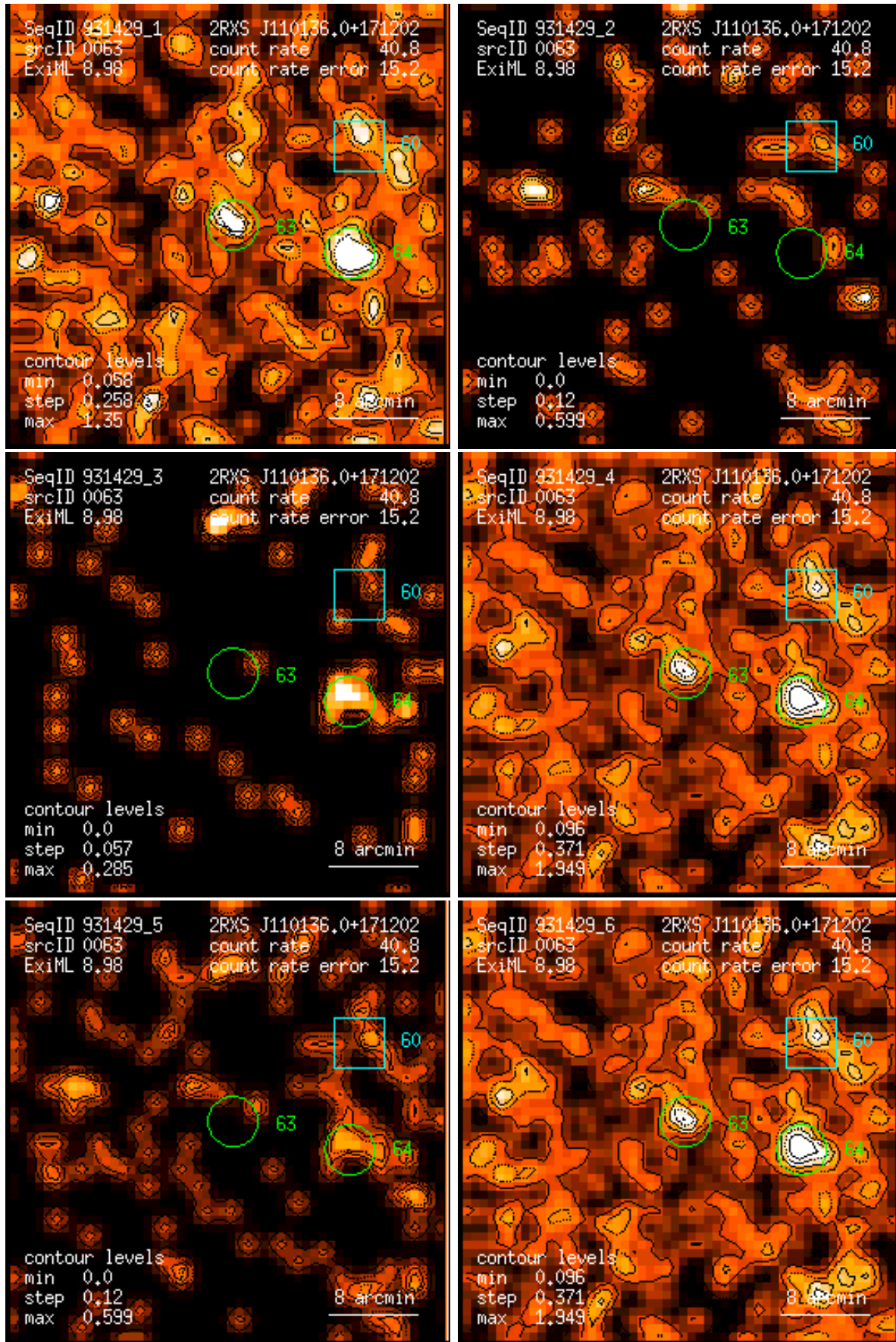
Figure 63: RASS 931429: detection 0063: band rate images, Gaussian filter: (1) PSPC channels 11 – 41, (2) 52 – 90, (3) 91 – 201, (4) 11 – 235, (5) 52 – 201, (6) 11 – 201. Broad band rates in counts/ks. Band rate contour levels in counts/ks/arcmin 2 .
