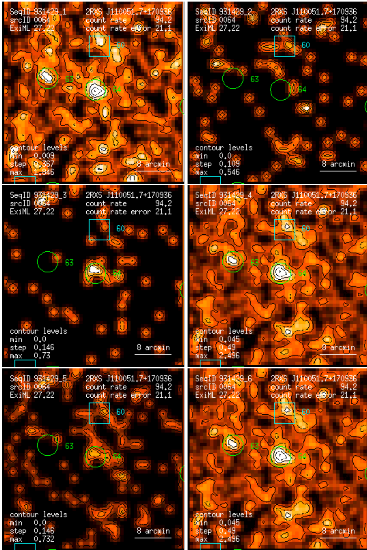
Figure 64: RASS 931429: detection 0064: band rate images, Gaussian filter: (1) PSPC channels 11 – 41, (2) 52 – 90, (3) 91 – 201, (4) 11 – 235, (5) 52 – 201, (6) 11 – 201. Broad band rates in counts/ks. Band rate contour levels in counts/ks/arcmin 2 .
