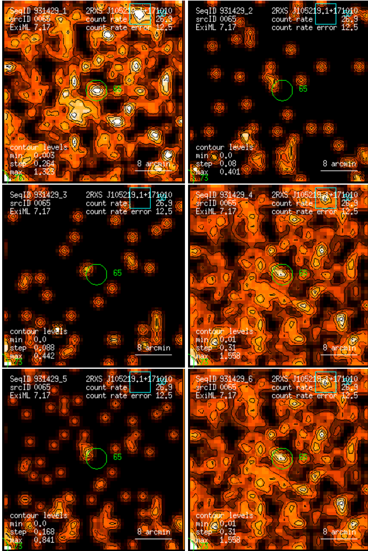
Figure 65: RASS 931429: detection 0065: band rate images, Gaussian filter: (1) PSPC channels 11 – 41, (2) 52 – 90, (3) 91 – 201, (4) 11 – 235, (5) 52 – 201, (6) 11 – 201. Broad band rates in counts/ks. Band rate contour levels in counts/ks/arcmin 2 .
