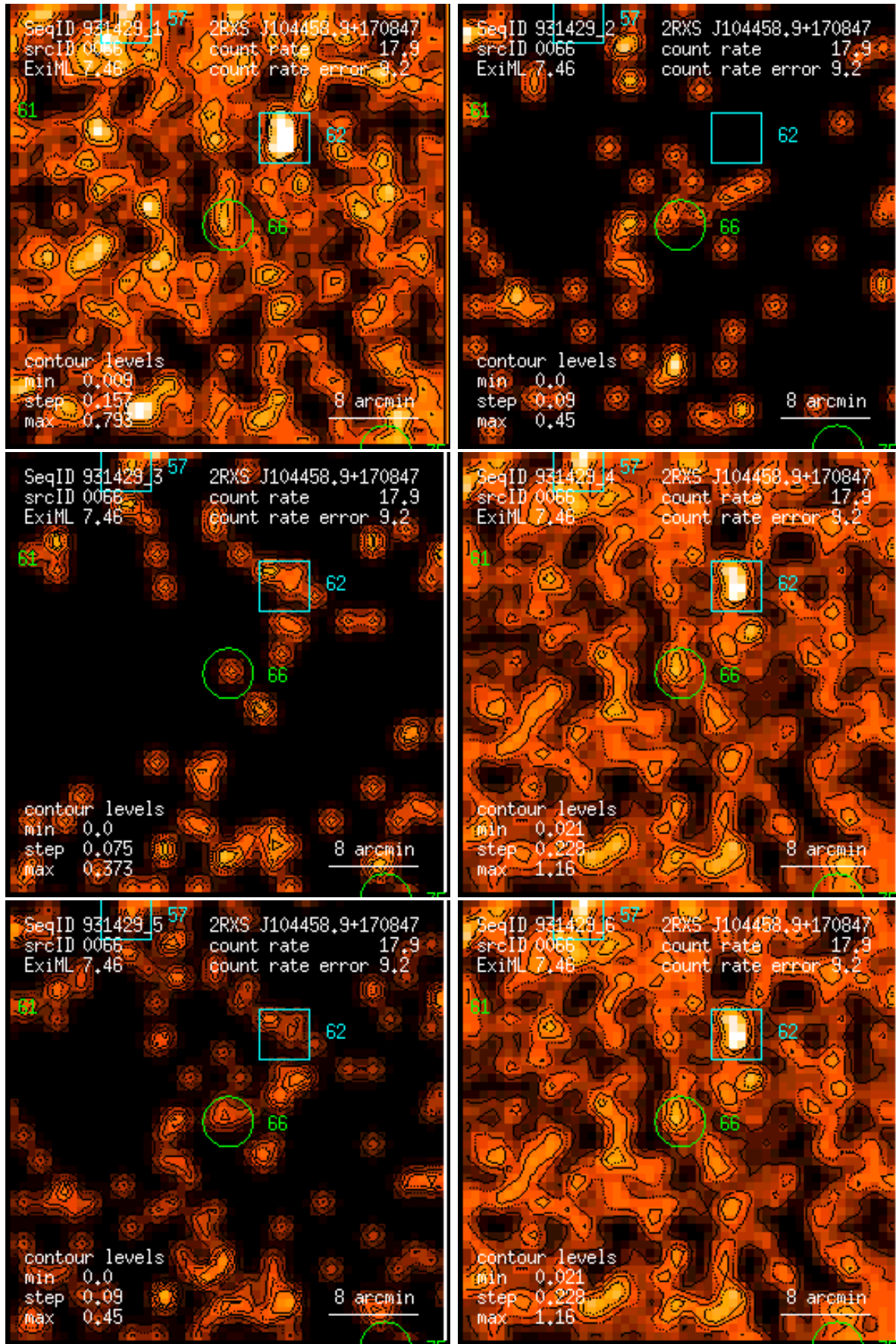
Figure 66: RASS 931429: detection 0066: band rate images, Gaussian filter: (1) PSPC channels 11 – 41, (2) 52 – 90, (3) 91 – 201, (4) 11 – 235, (5) 52 – 201, (6) 11 – 201. Broad band rates in counts/ks. Band rate contour levels in counts/ks/arcmin 2 .
